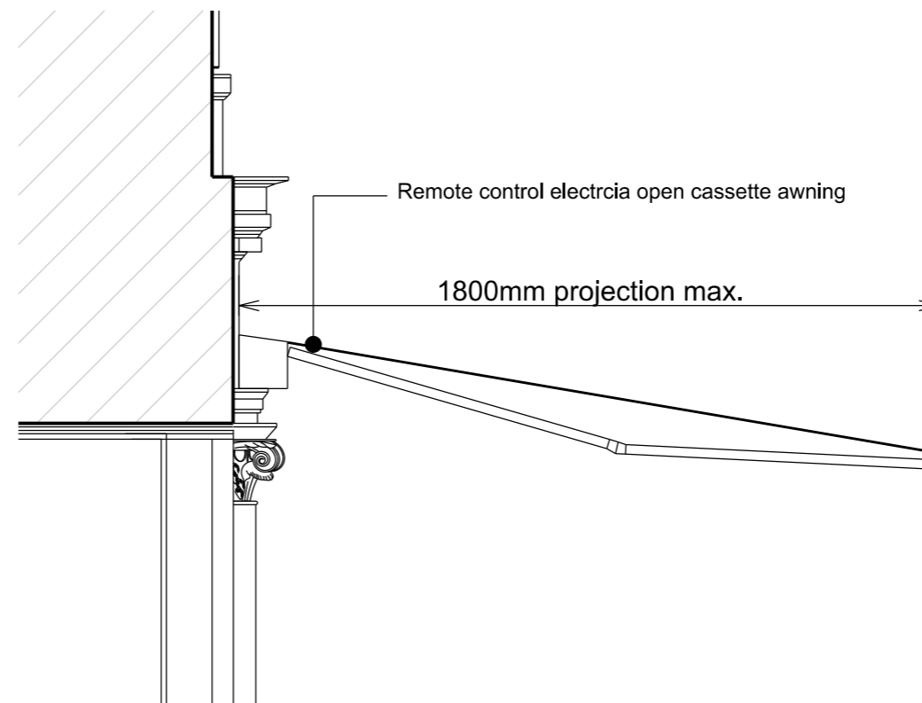
Awning side elevation (not to scale)
