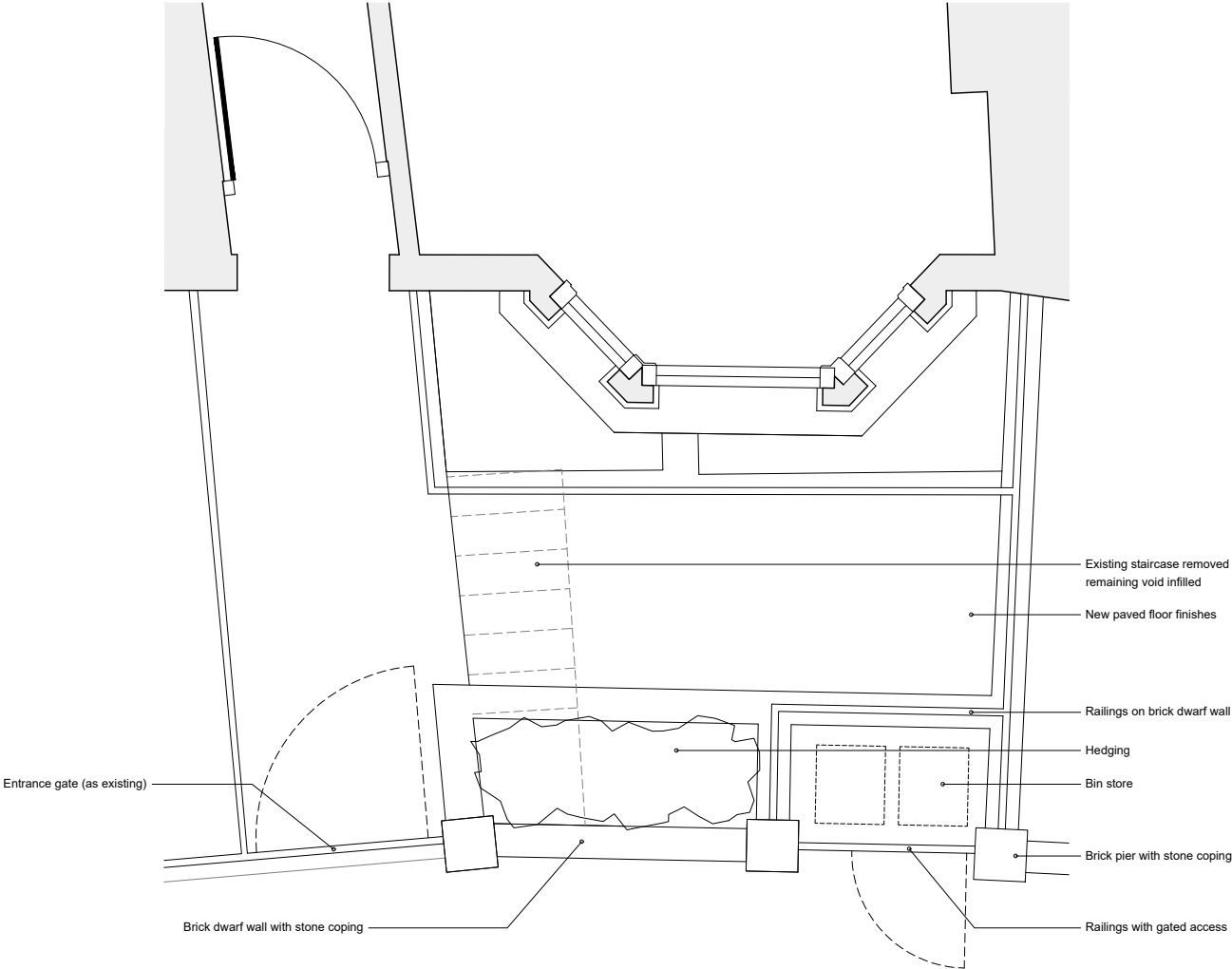
ENTRANCE WAY PLAN @1:50
