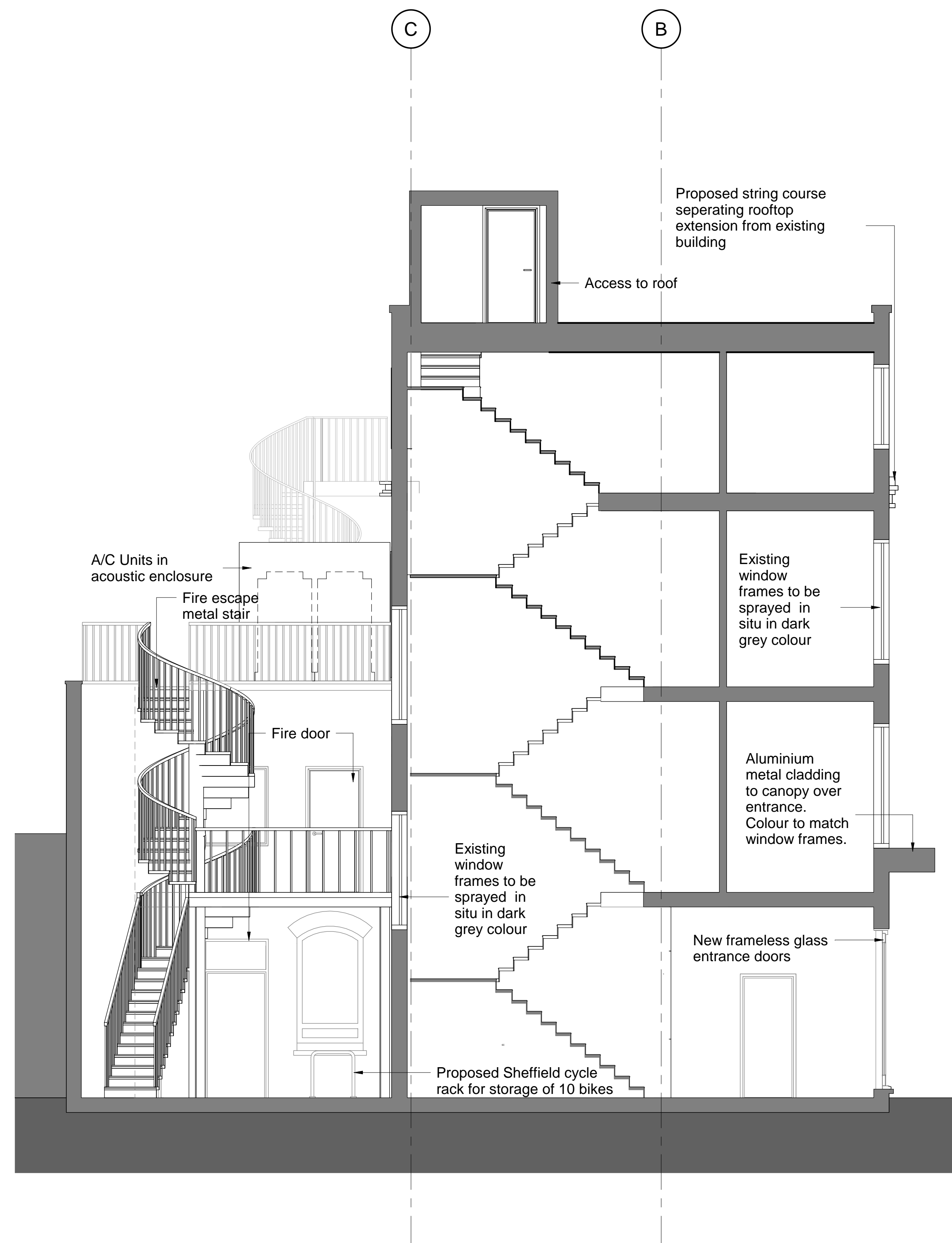
Proposed Section 1 : 50 @ A1 _ 1:100 @ A3
