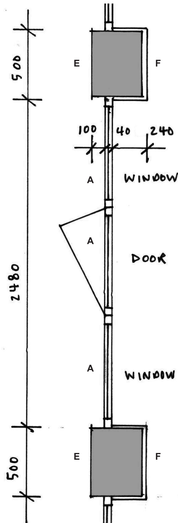
SECTION BB EXISTING
