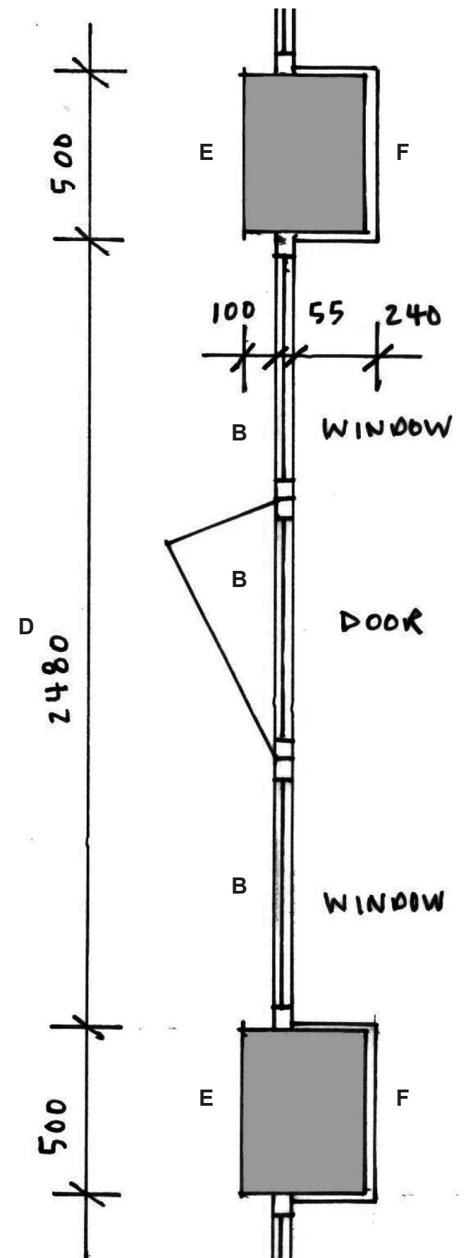
SECTION BB PROPOSED
