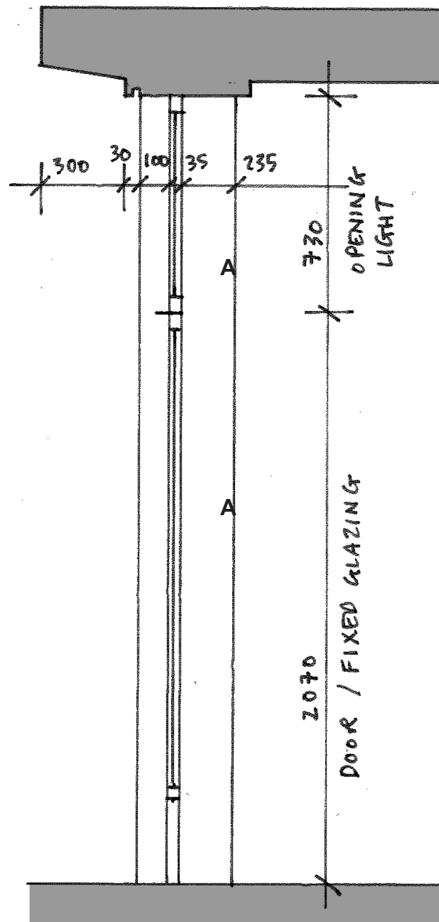
SECTION AA EXISTING
