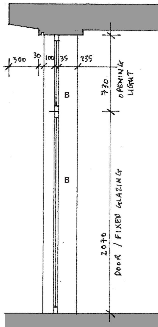
SECTION AA PROPOSED
