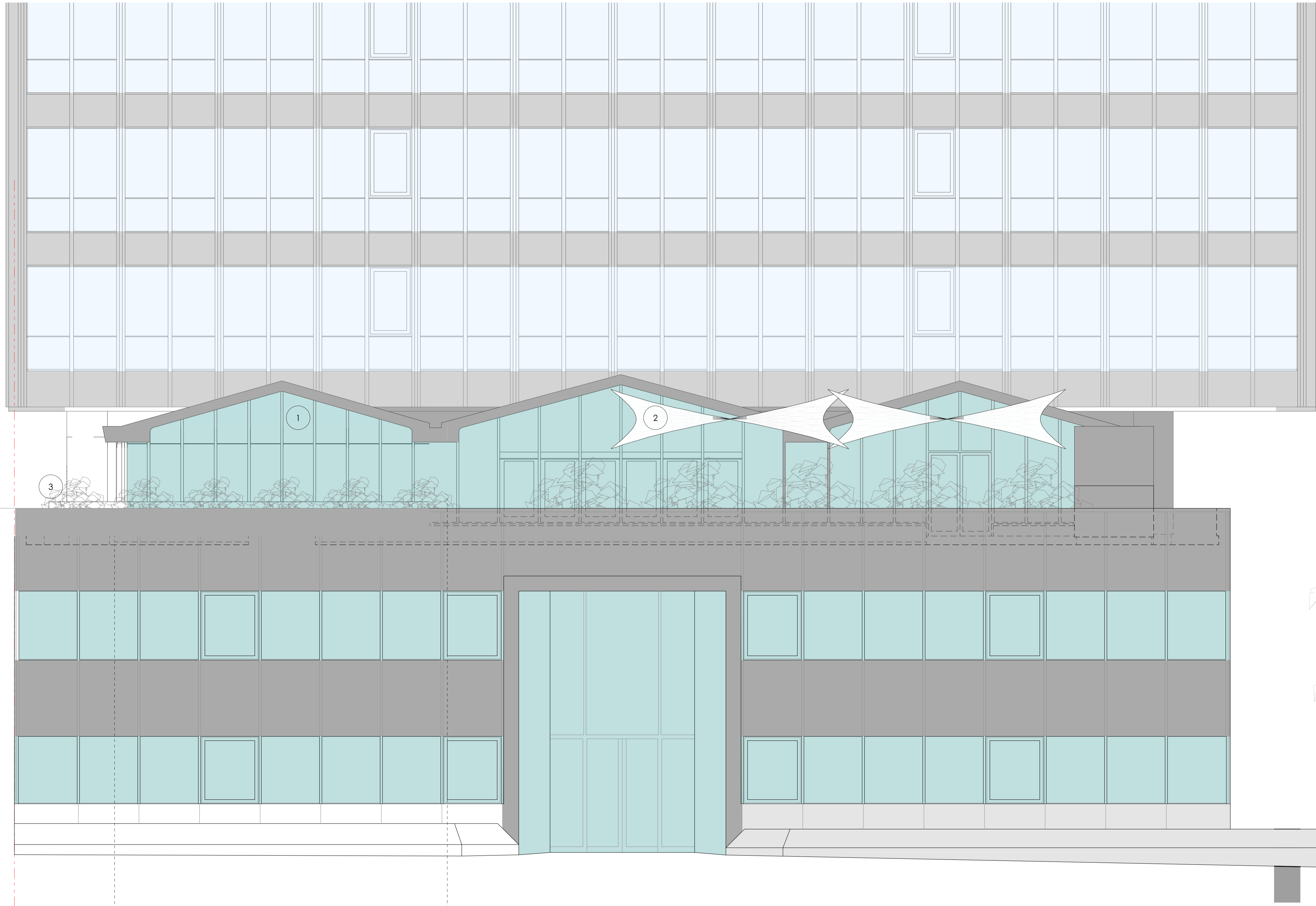
South elevation
