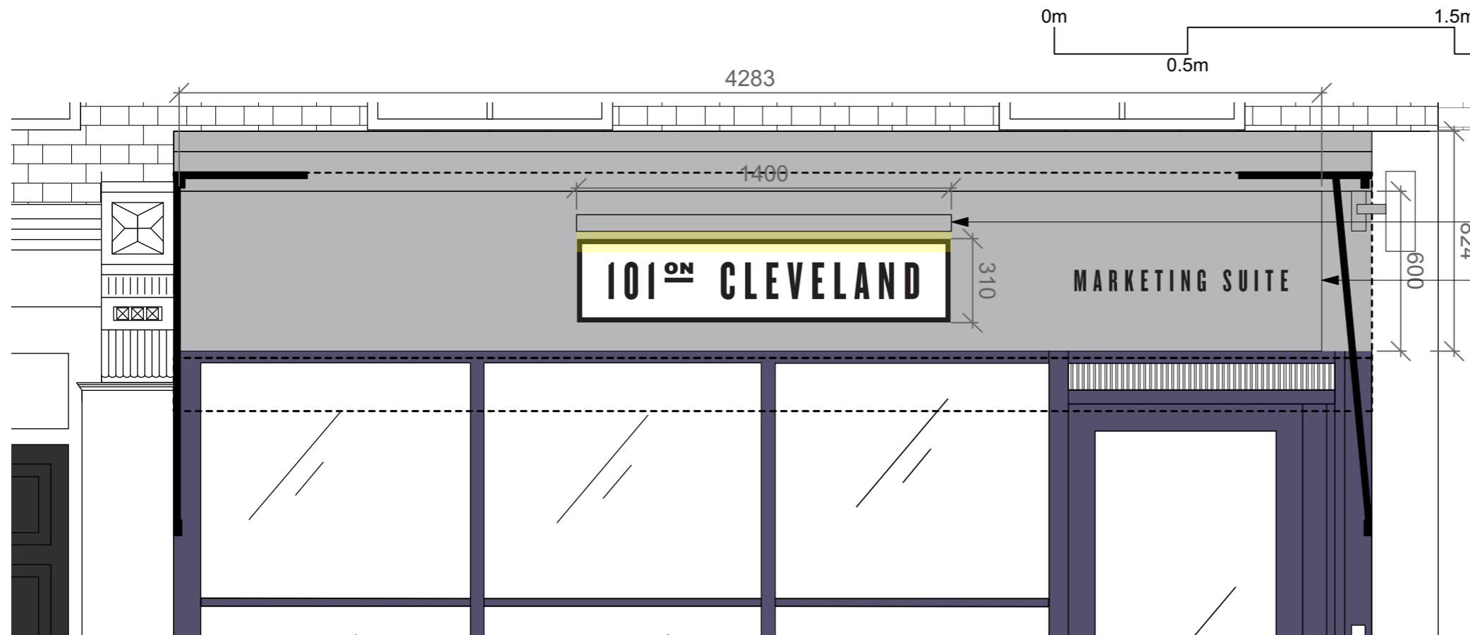
1 Awning Design Detail (Retracted) Scale: 1:20
