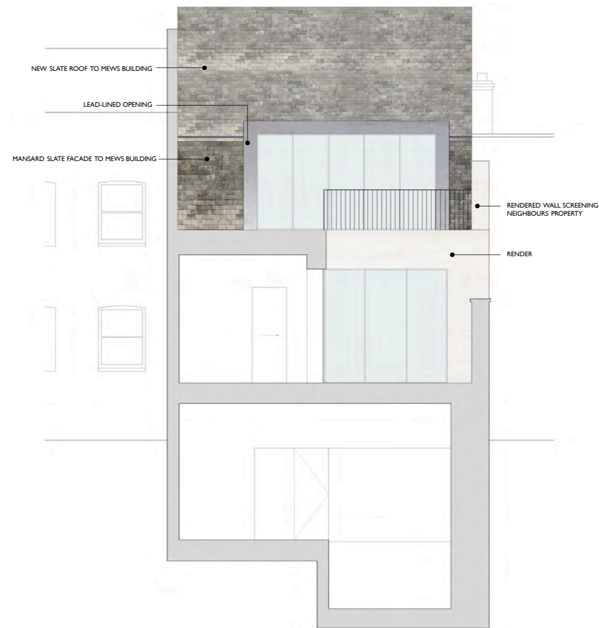
WEST ELEVATION OF PROPOSED MEWS MATERIAL STUDY
