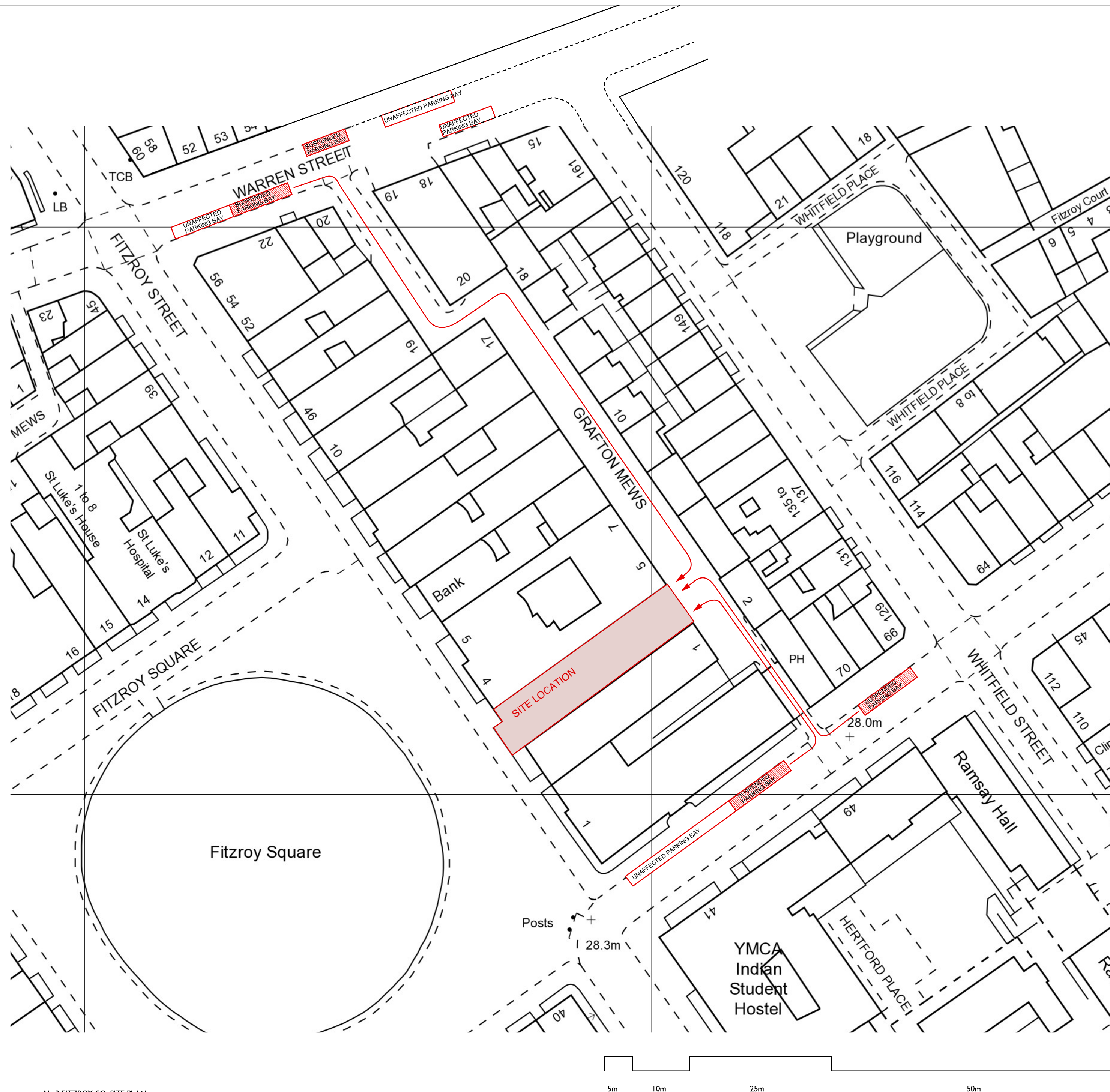
No.3 FITZROY SQ. SITE PLAN
