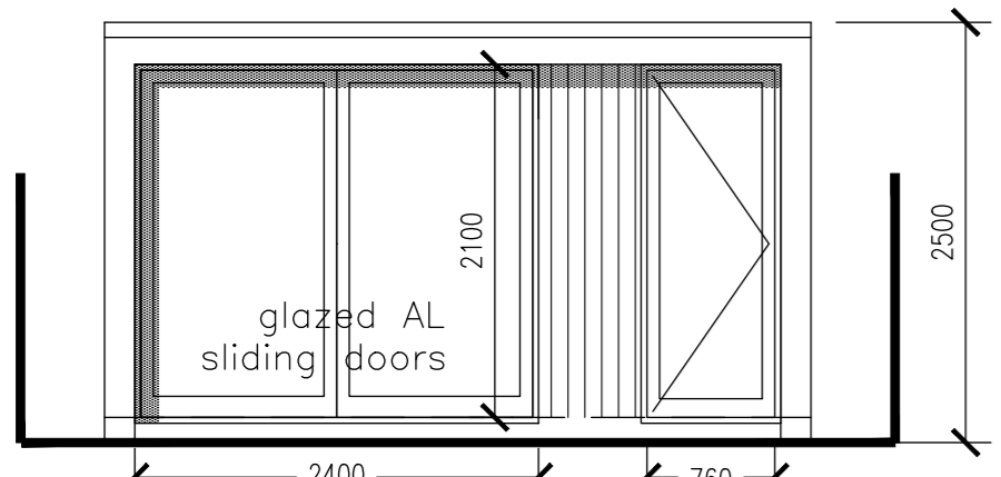
FRONT (NE) ELEVATION
