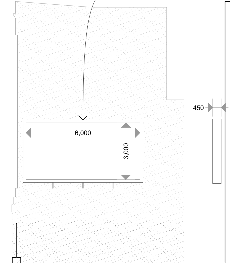
Existing South East Elevation
