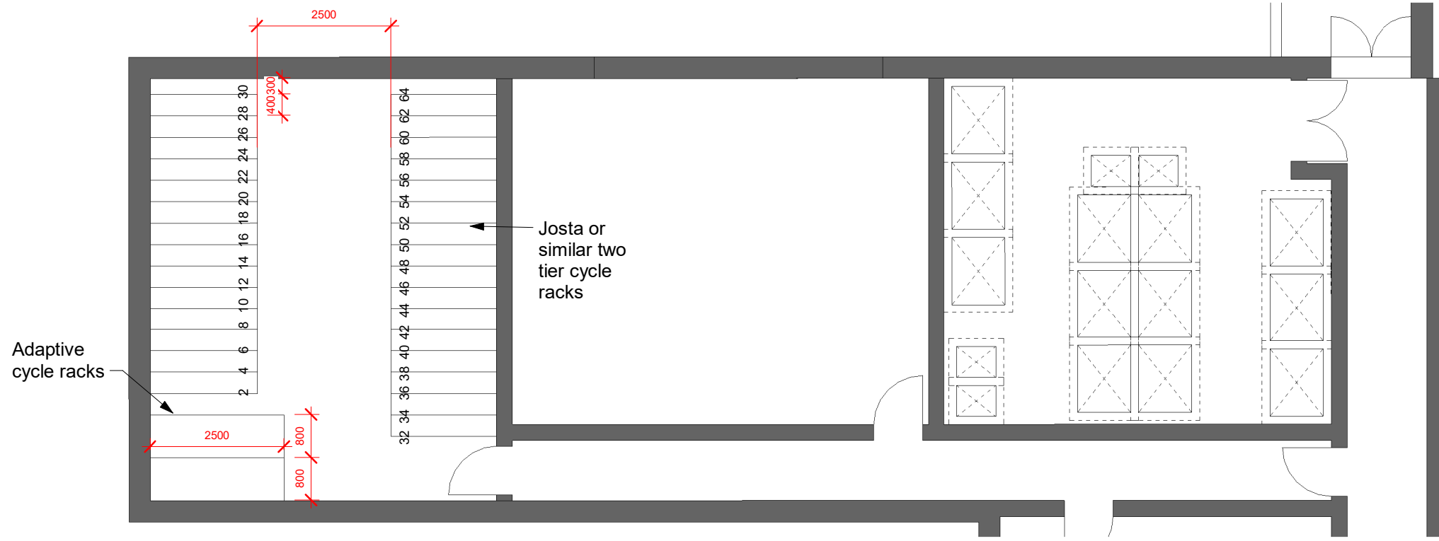
1 Cycle store plan - Private sale 1 1 : 100
