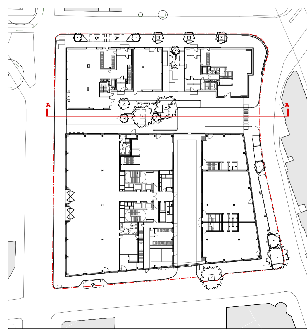
Key Plan 1:750 @ A1
