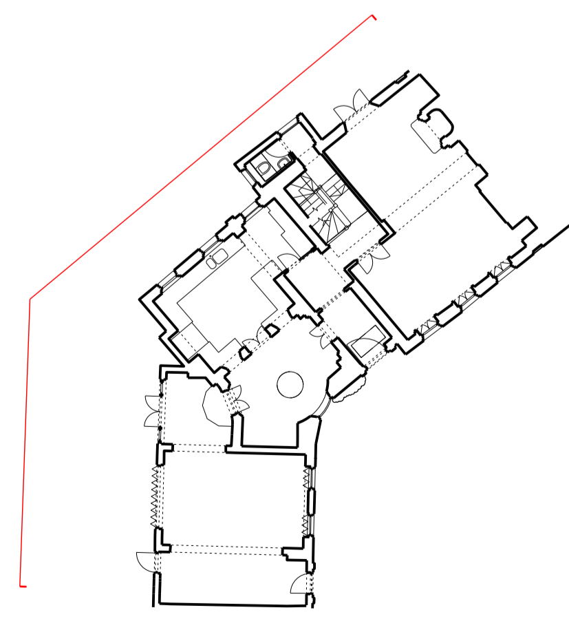
2 1:200 EXISTING GROUND FLOOR KEYPLAN
