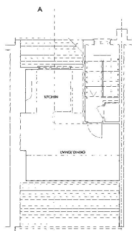
EXISTING THIRD FLOOR PLAN
