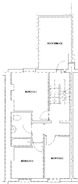
EXISTING SECOND FLOOR PLAN
