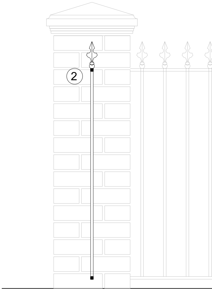
Section Detail
