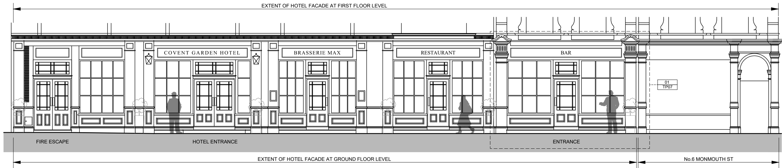
1 EXISTING ELEVATION
