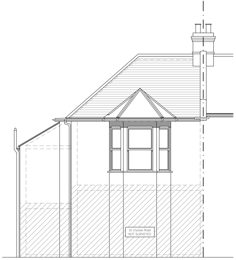
FRONT ELEVATION
