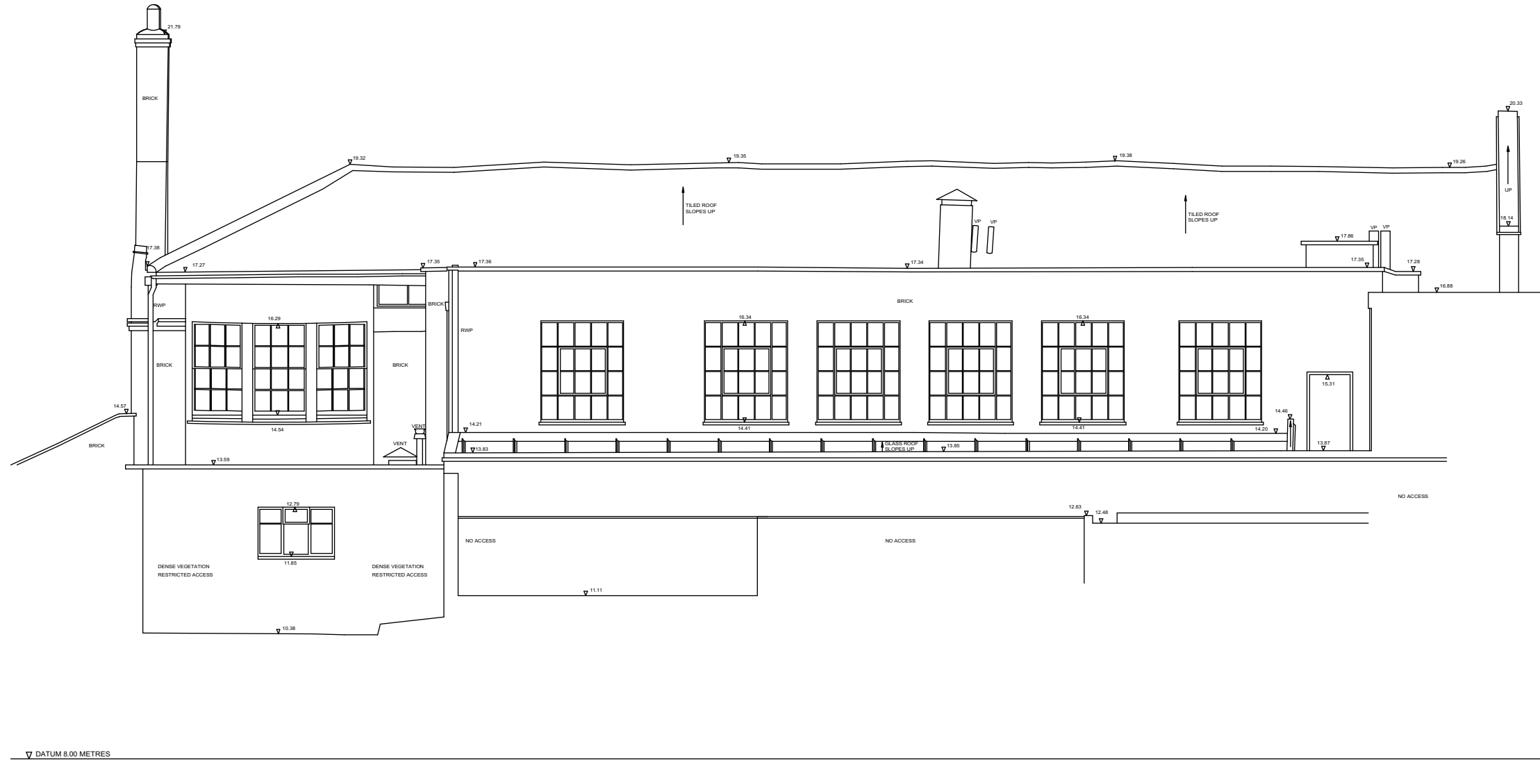
REAR ELEVATION
