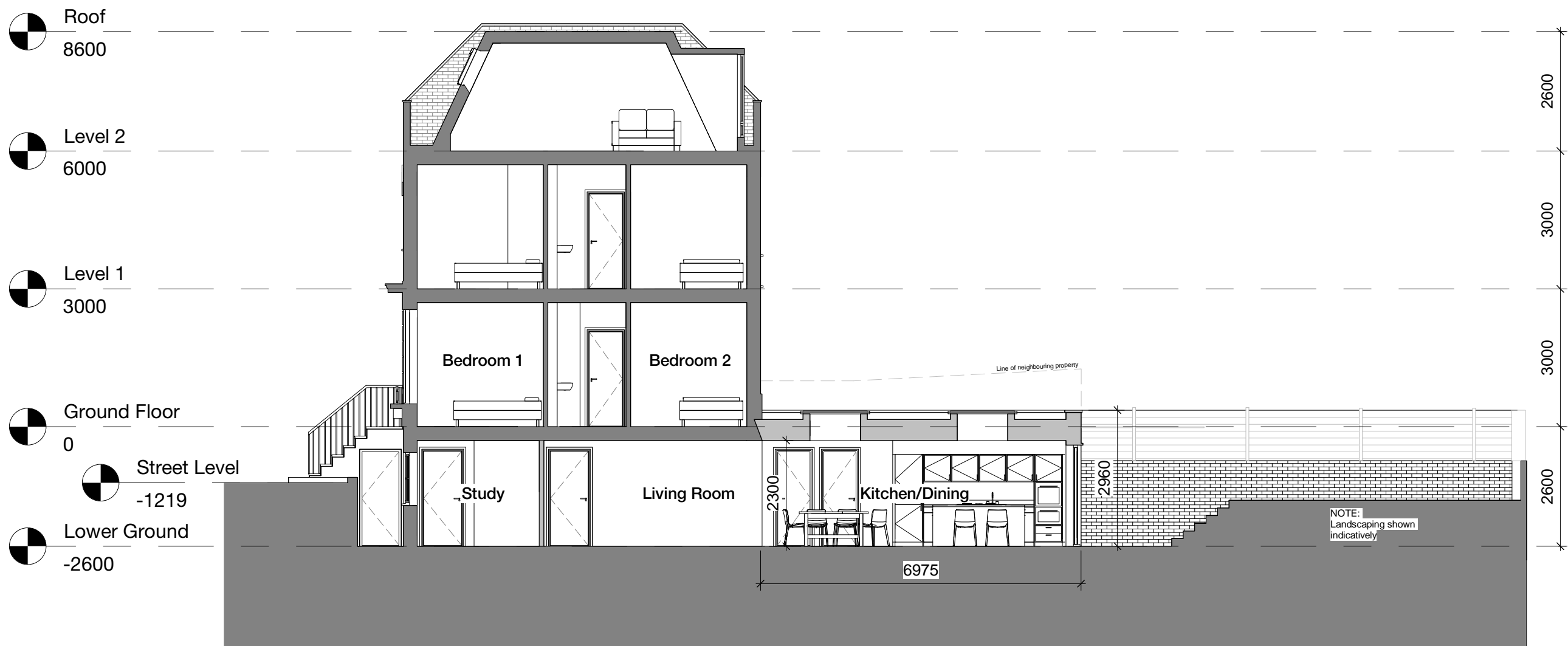
Proposed Section A-A 1 : 100
