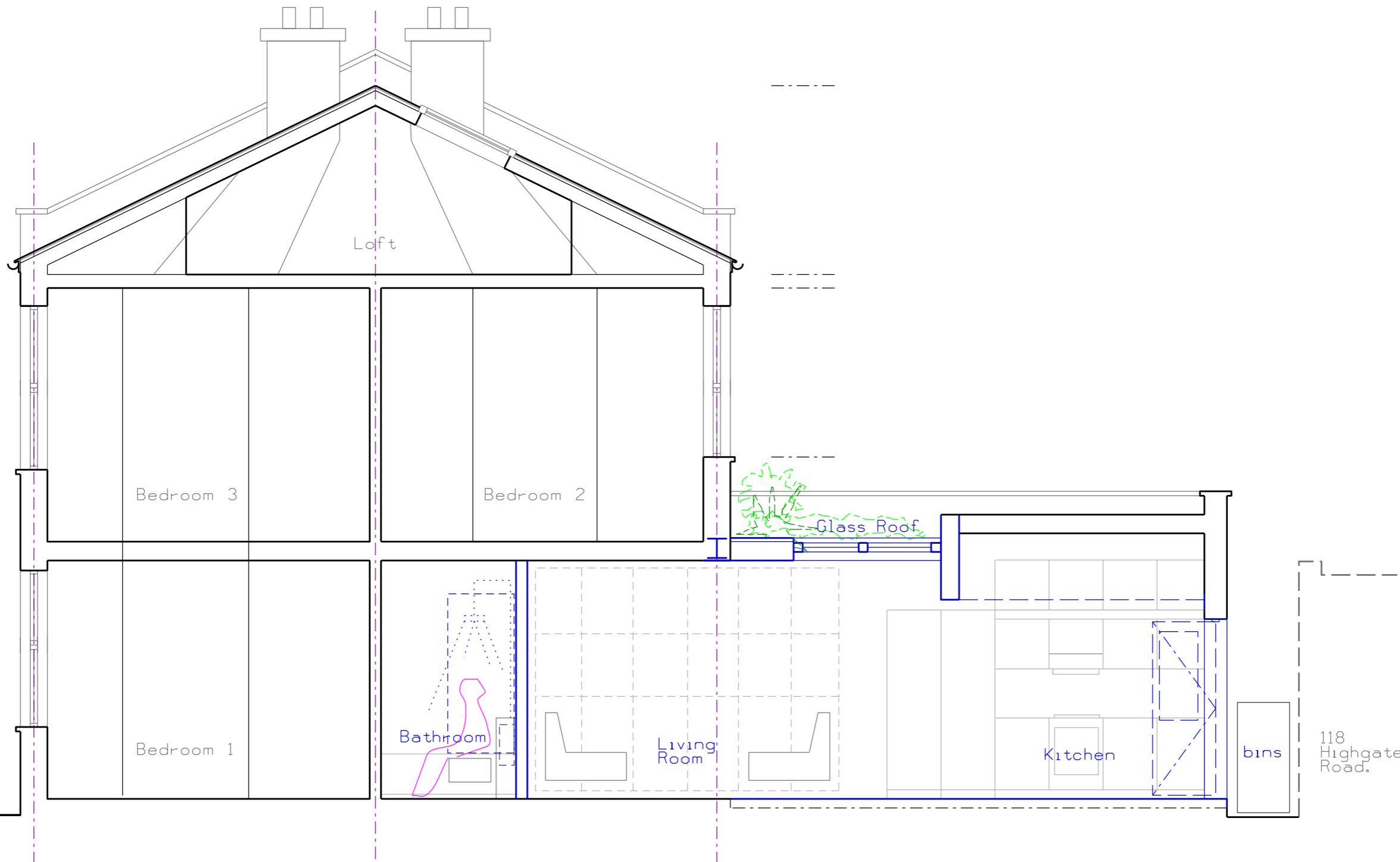
Proposed Section AA 1:50@A3
