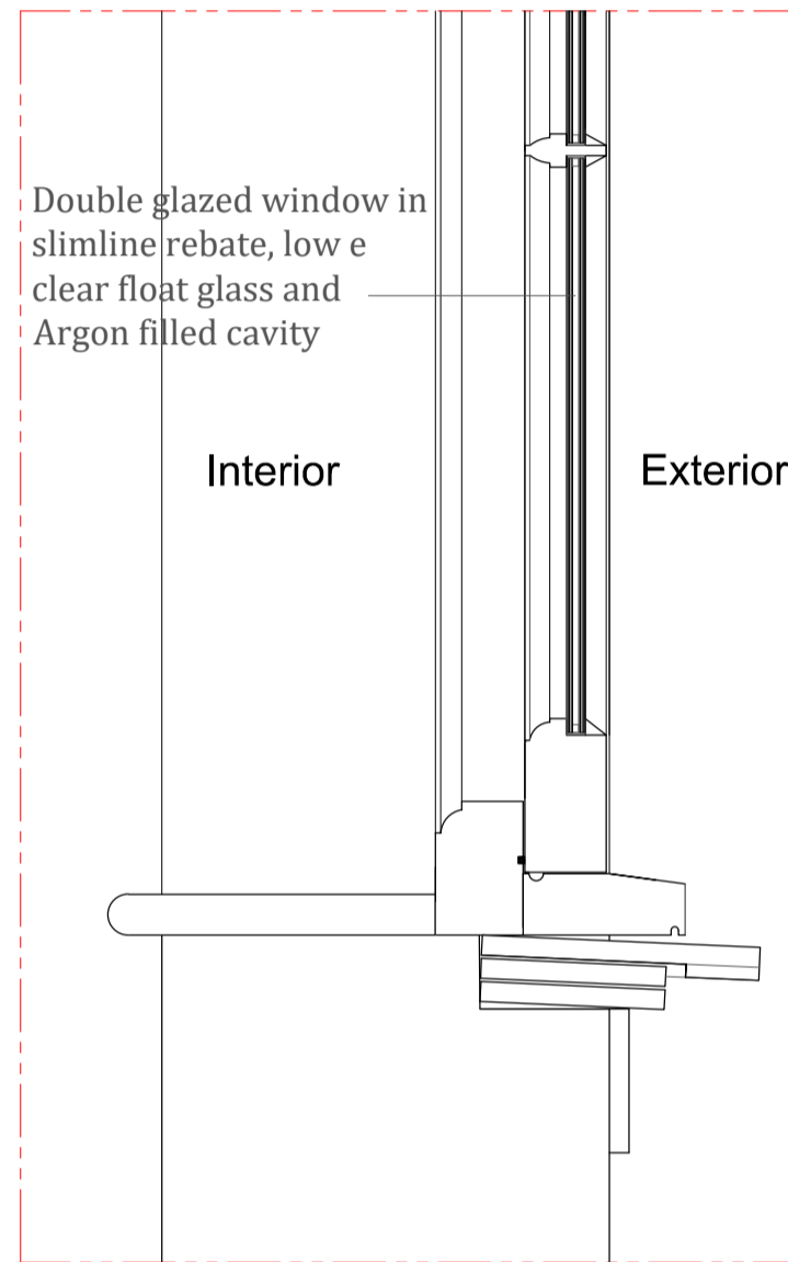
Section - details
