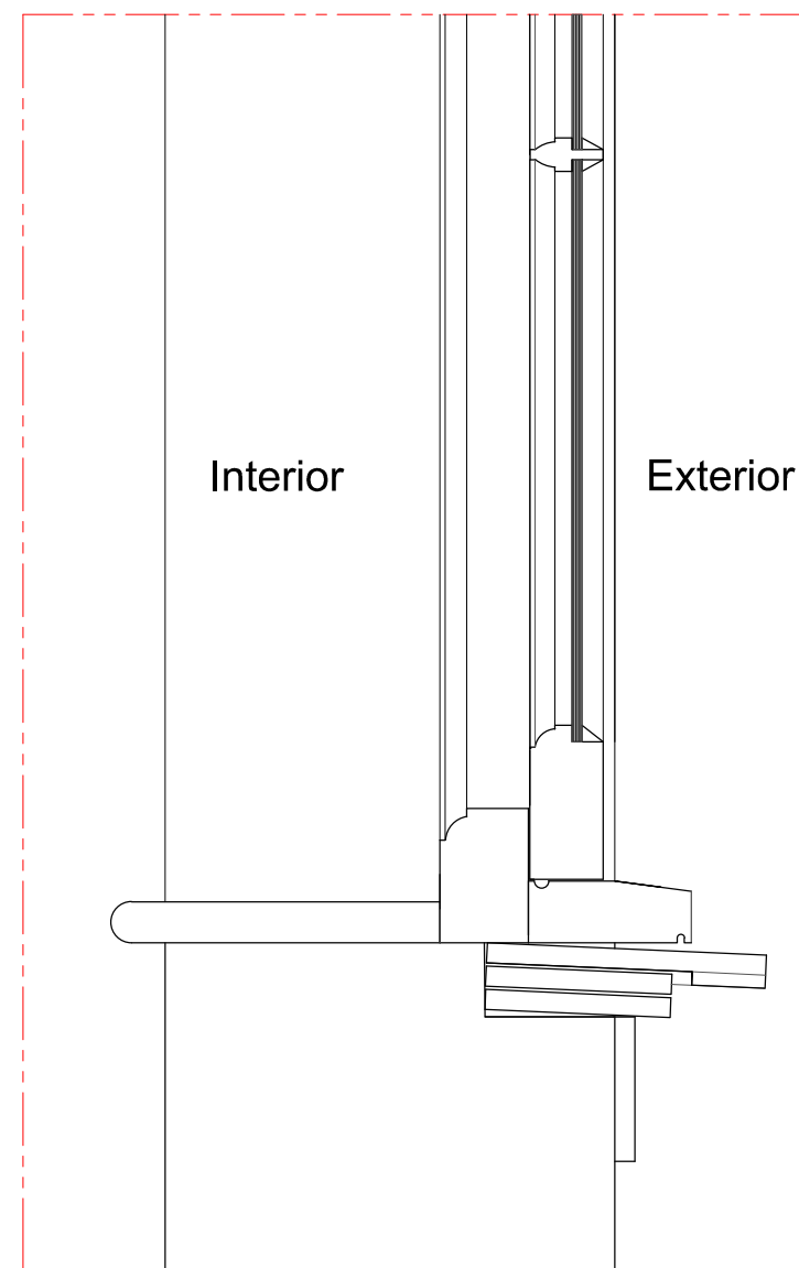
Section - details
