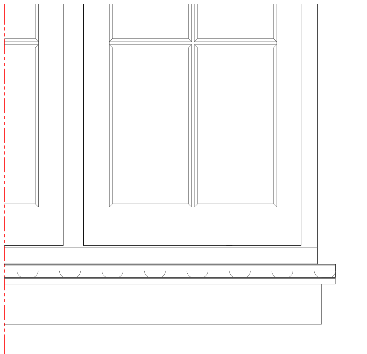
Exterior Elevation - details
