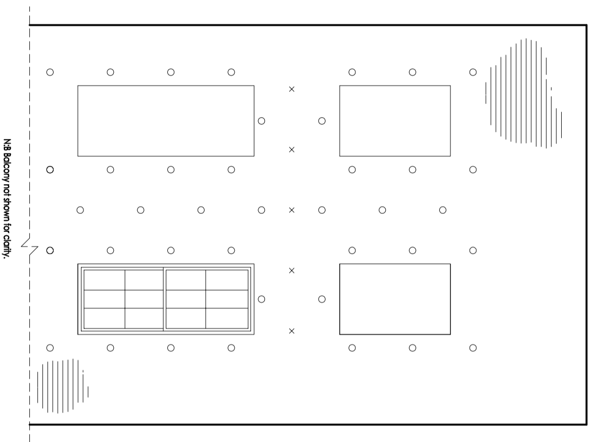
Proposed Helifix Repair Front Elevation (Part of)
