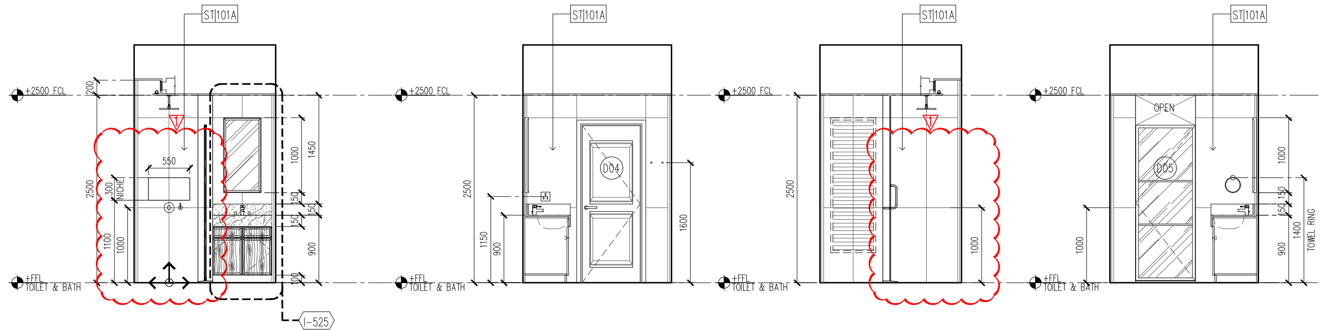
1 ELEVATION 105-E8 1:50
