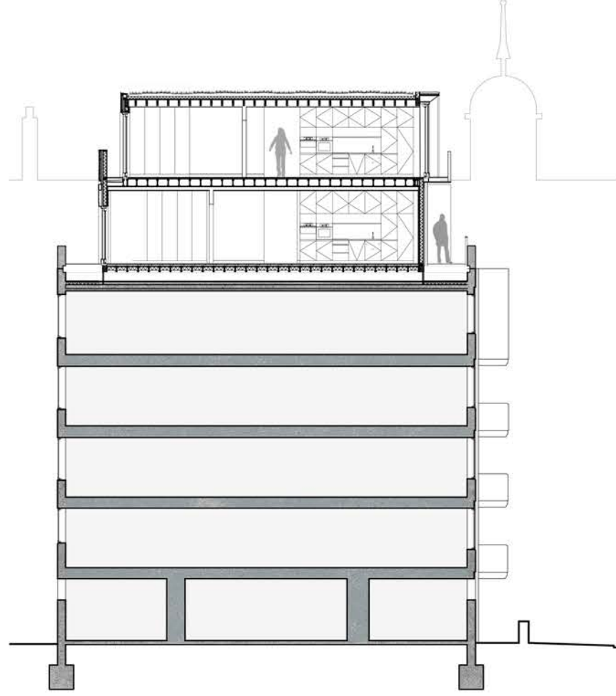
3 117 PROPOSED SECTION A - A 1:200 @A3
