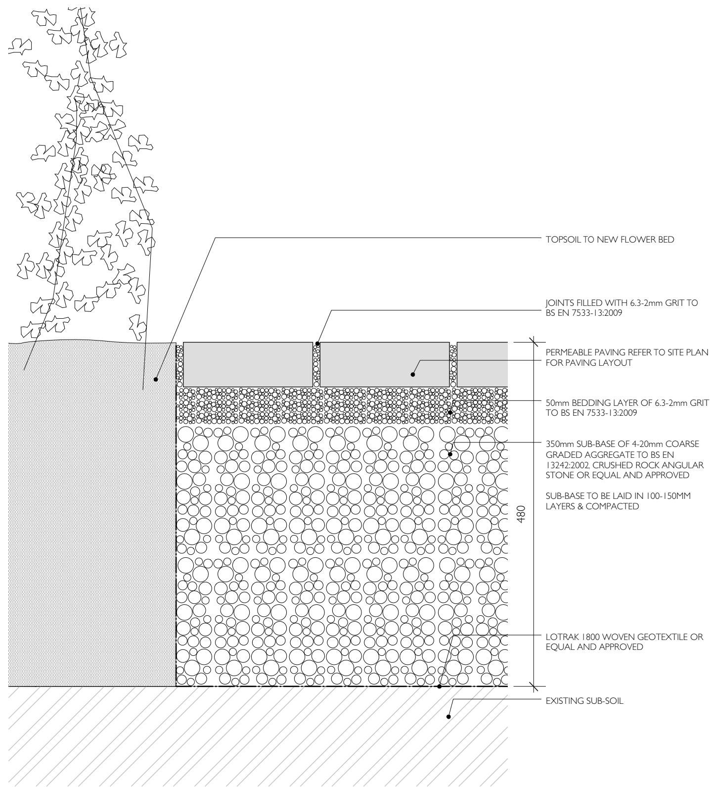
TYPICAL PAVING DETAIL SECTION SCALE 1:5 @A3
