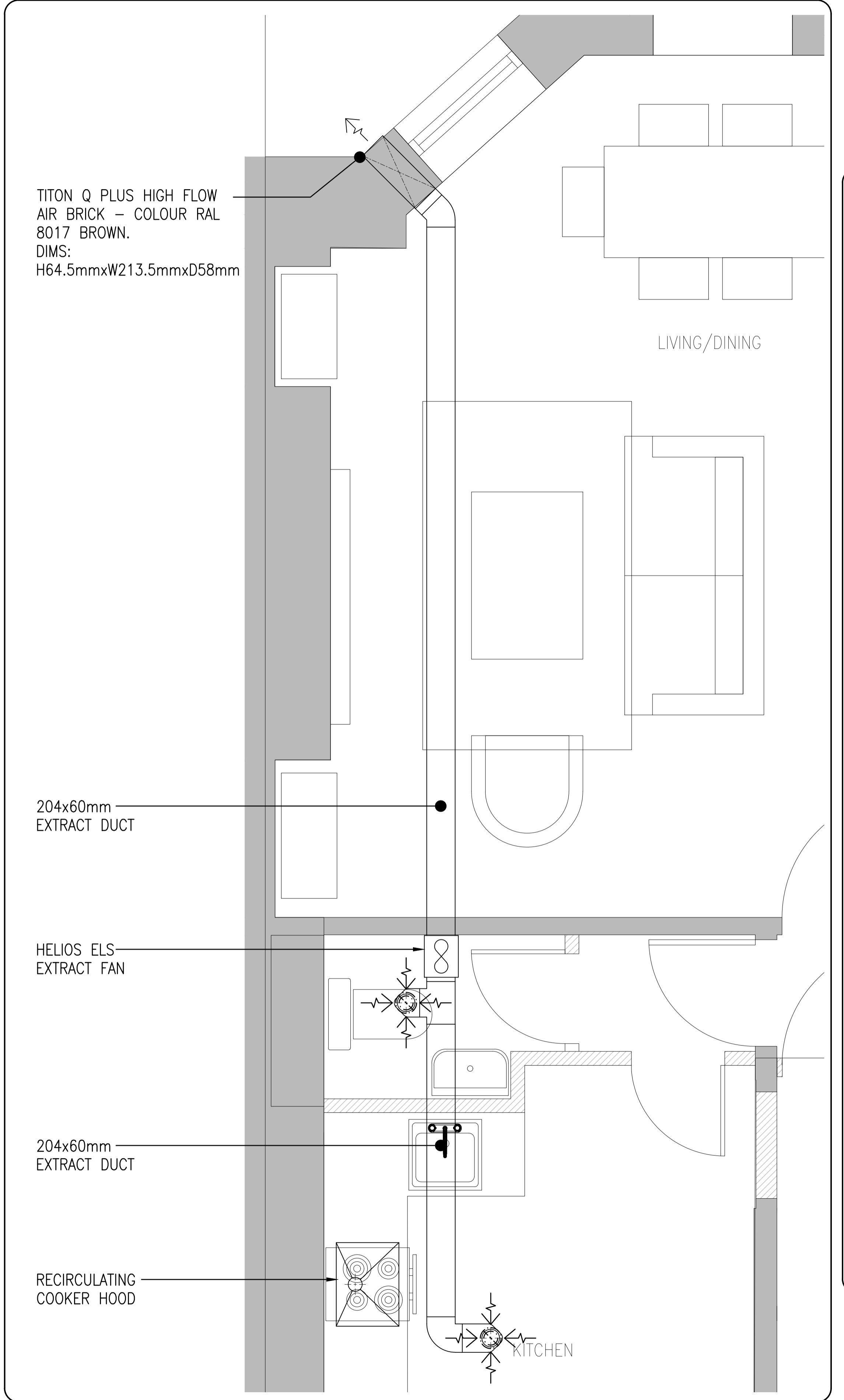
SECOND FLOOR DUPLEX DETAIL
