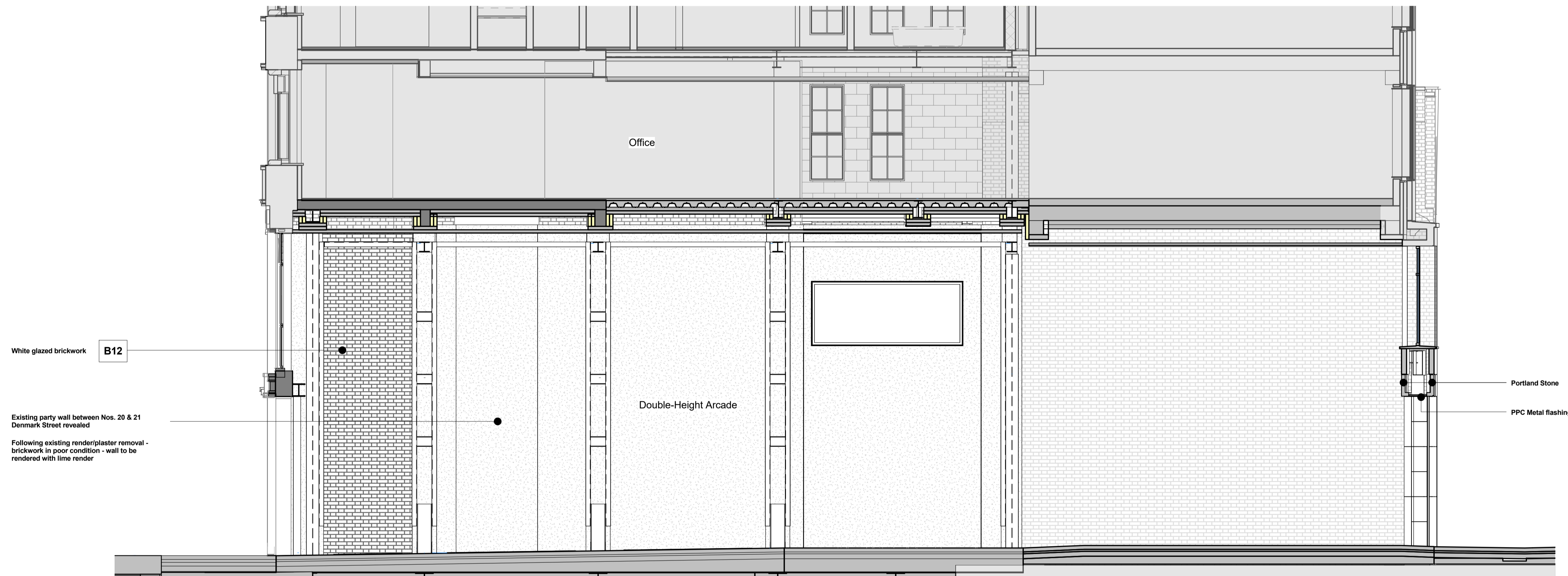
1 No. 21 Denmark Street Detail section through Double Height Arcade Space Scale: 1 : 50
