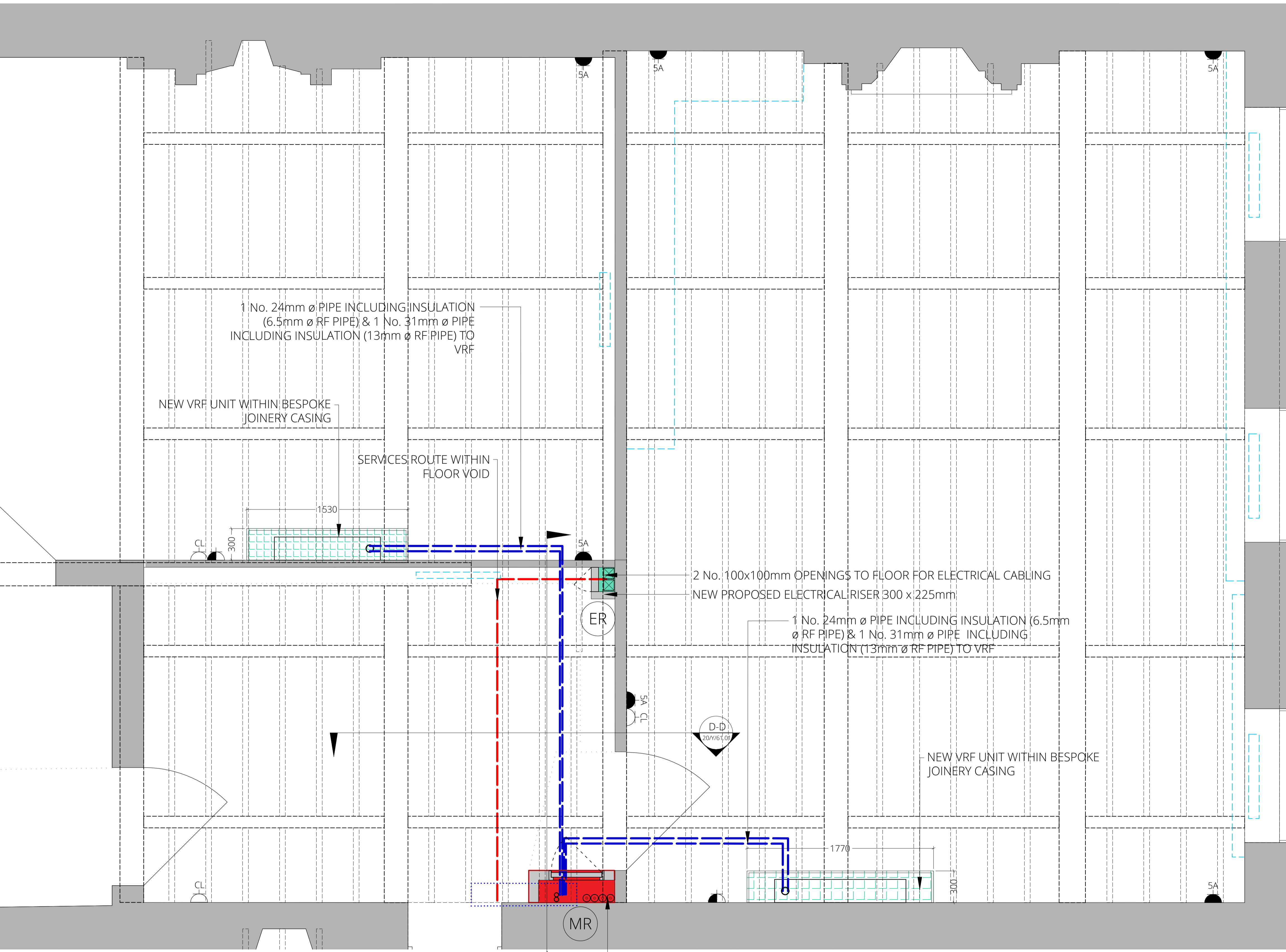
ABA's Servicing Strategy Drawing
