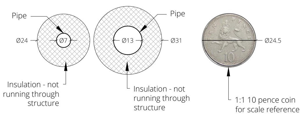
1:1 @ A1 RF PIPEWORK SIZES
