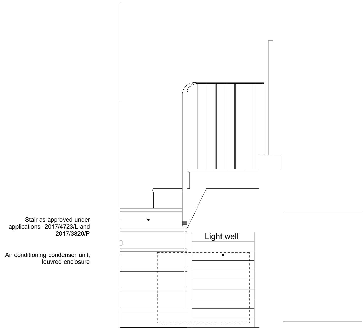
Stair Elevation
