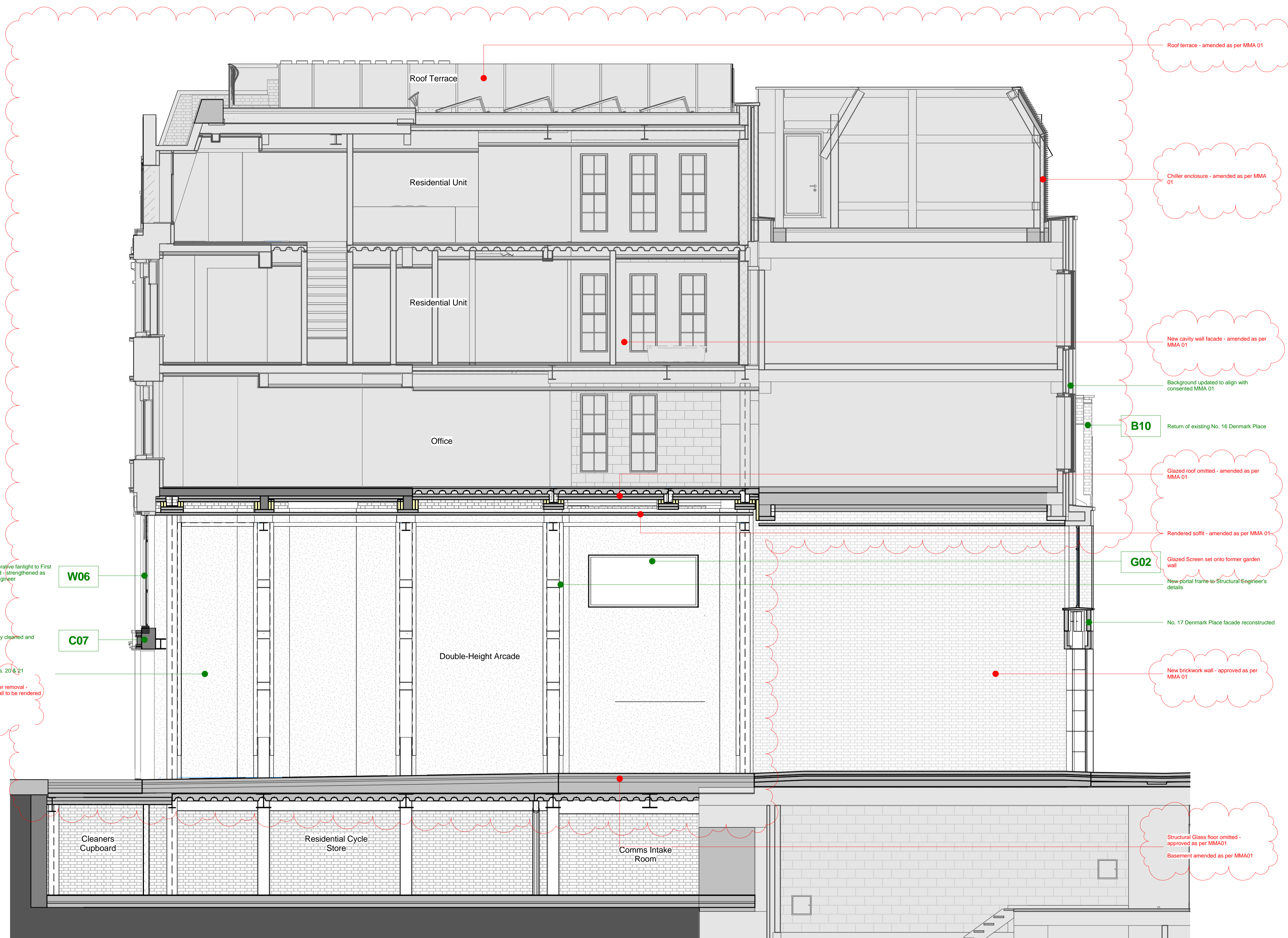
1 No. 20 Denmark Street Detail section through Double Height Arcade Space Scale: 1 : 50
