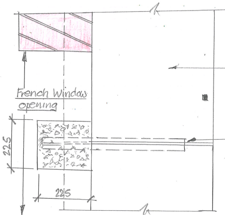
PLAN (1:10)
