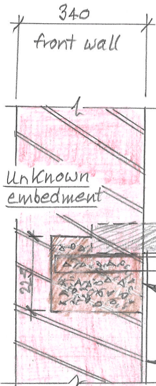
SECTION (1:10)
