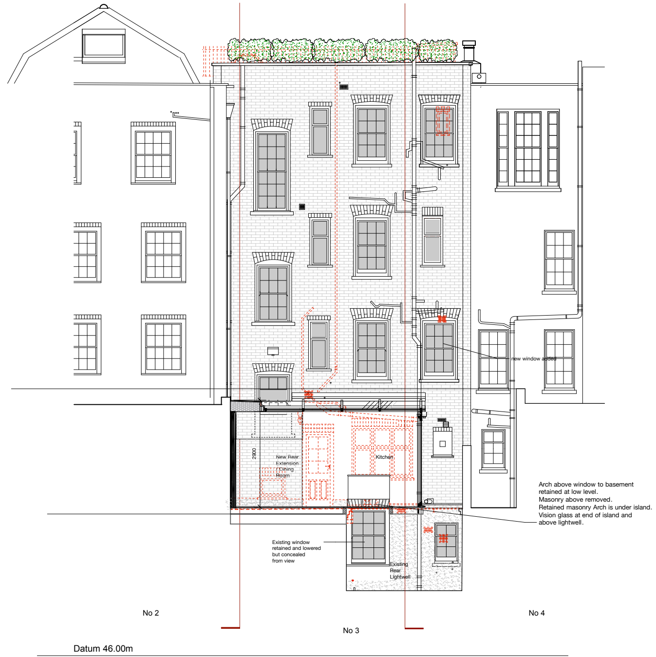
2 DEMOLITION REAR ELEVATION 1:50 @A1
