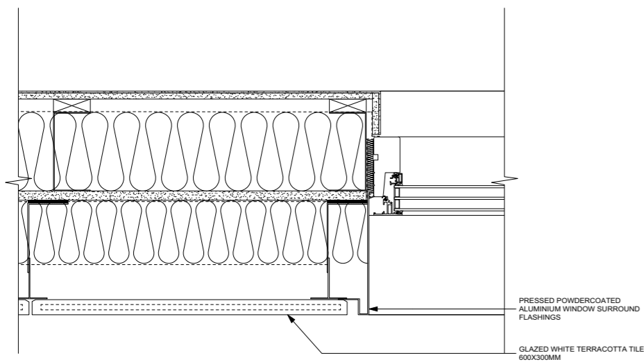
2 WINDOW JAMB DETAIL Scale: 1:5
