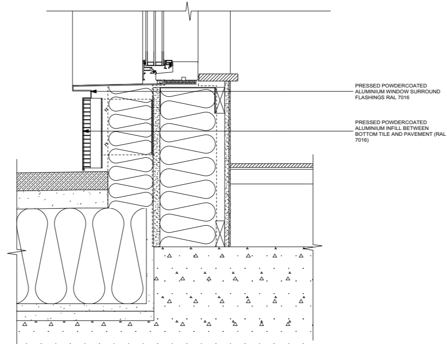
3 PLINTH/CILL DETAIL Scale: 1:5
