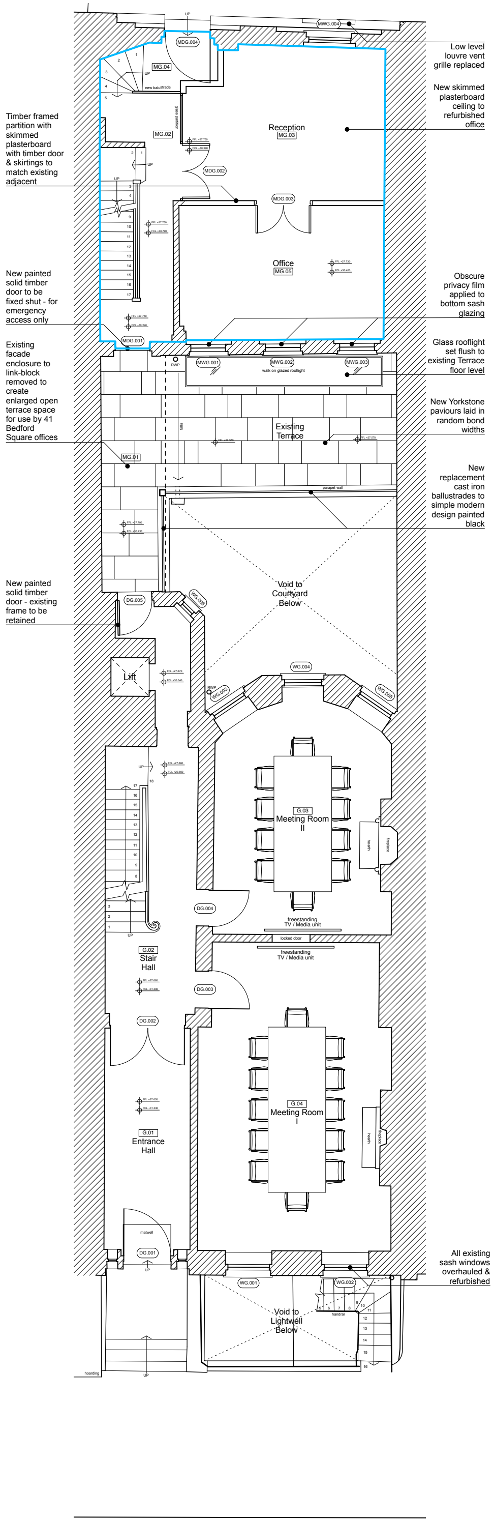
1 Proposed Ground Floor Plan PL_012 Scale 1:100 @ A3
