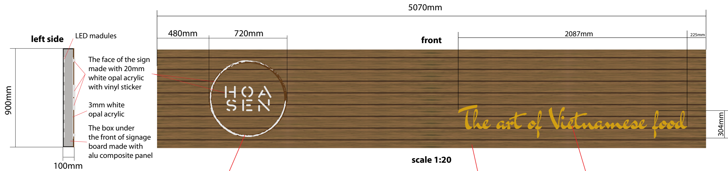
1. Logo illuminated by LED with 'halo' effect
