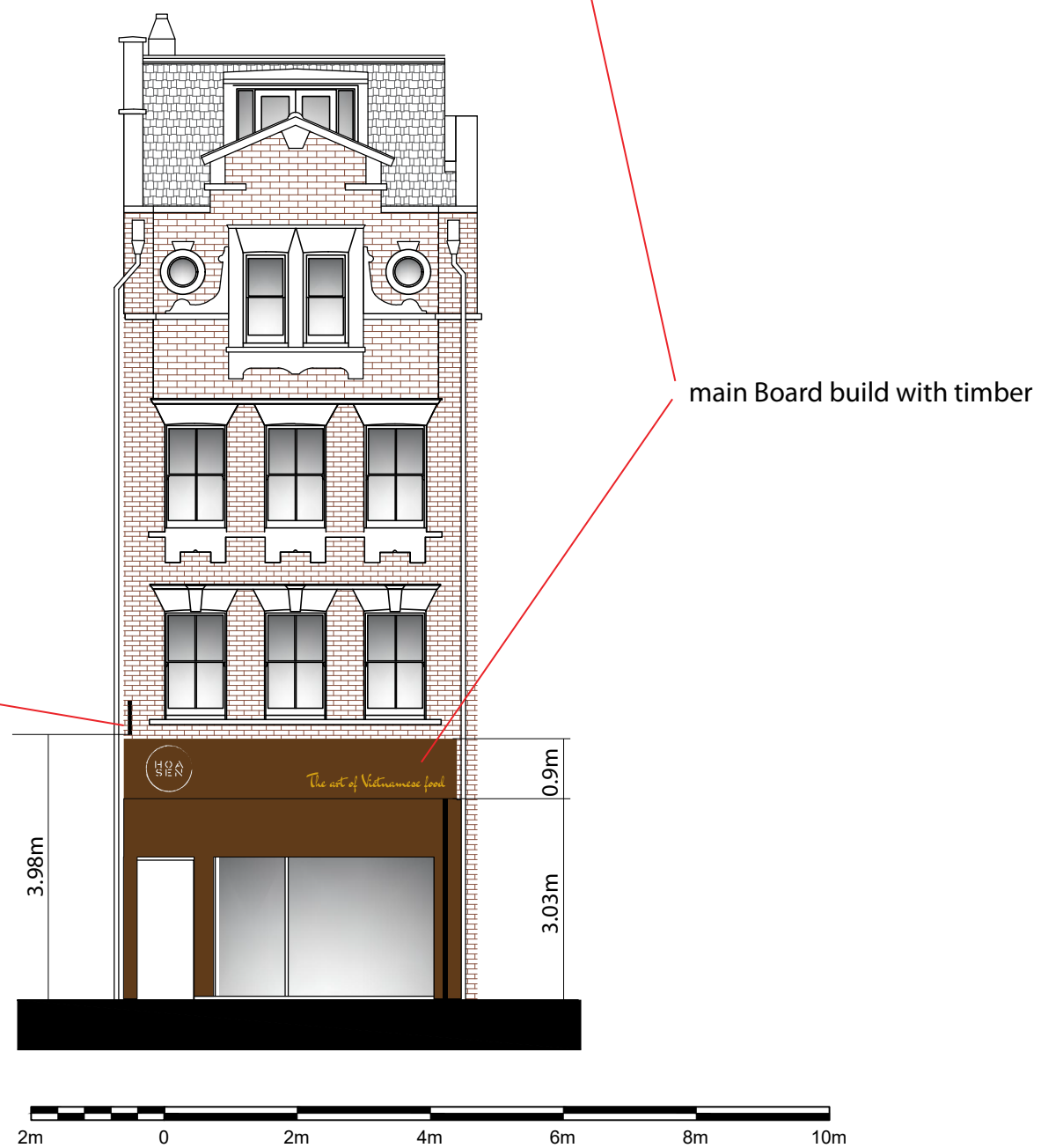
2. Solgan 'The art of vietnamese food' made with 10mm pvc foam painted to silk gold, fitted by pins and glue
