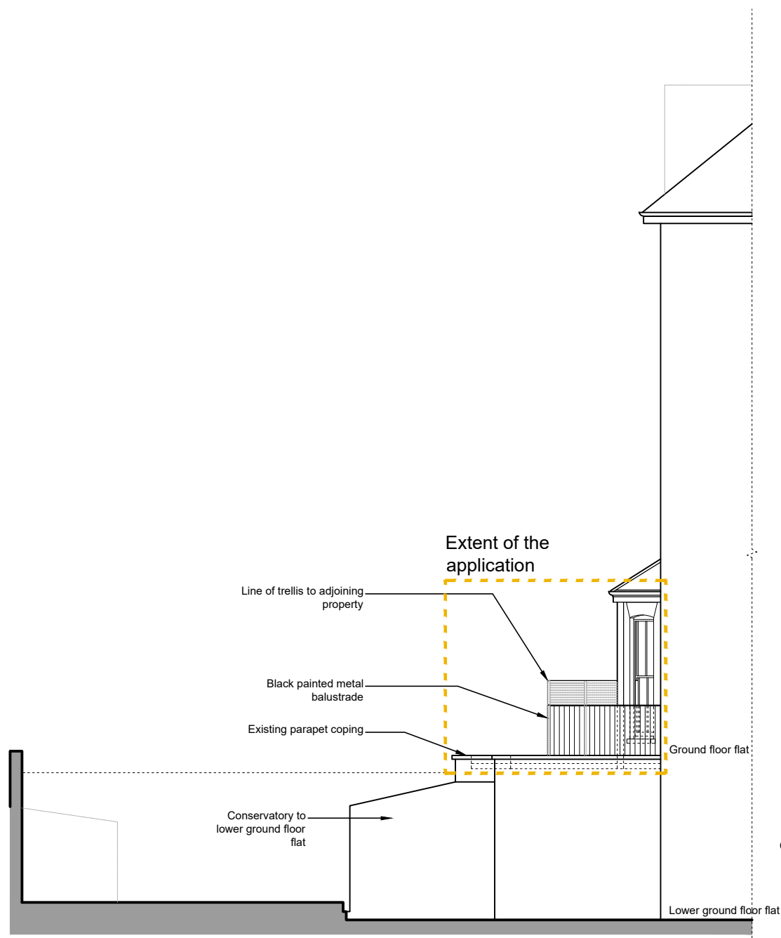
Side Elevation
