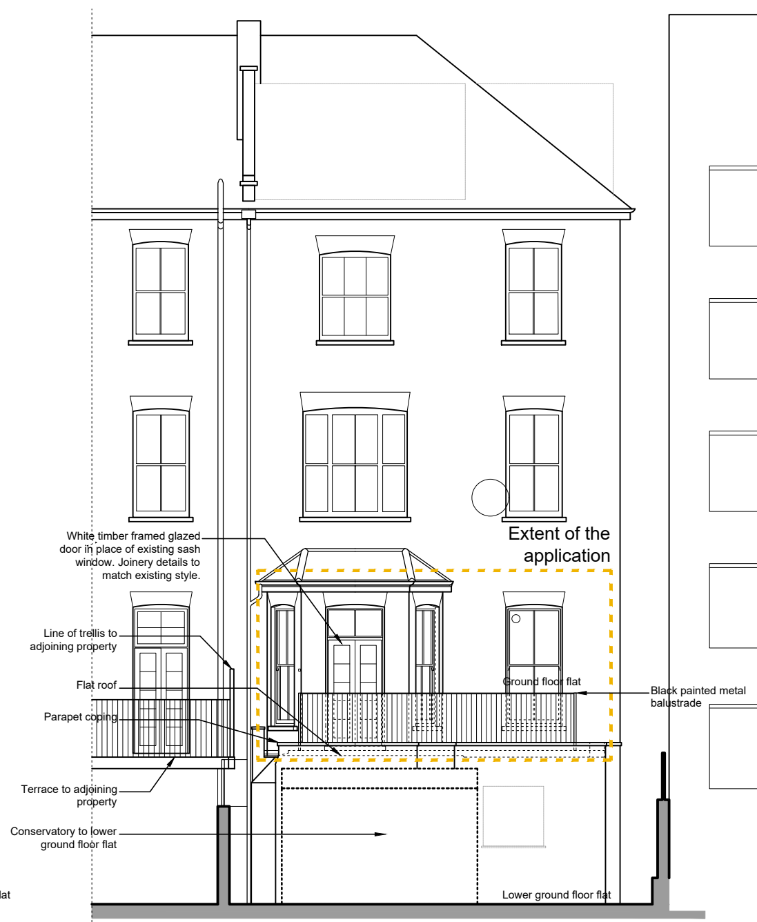
Rear Elevation
