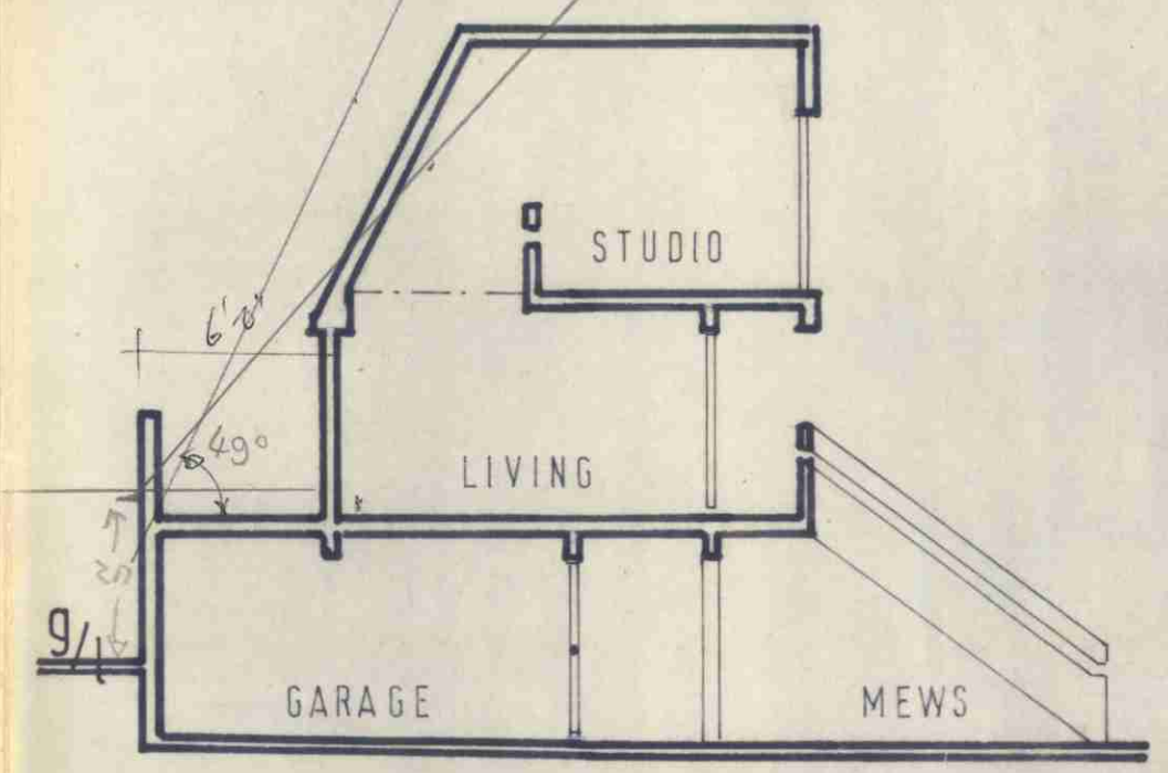
SECTION [LIVING ROOM ONLY WITH GALLERY]
