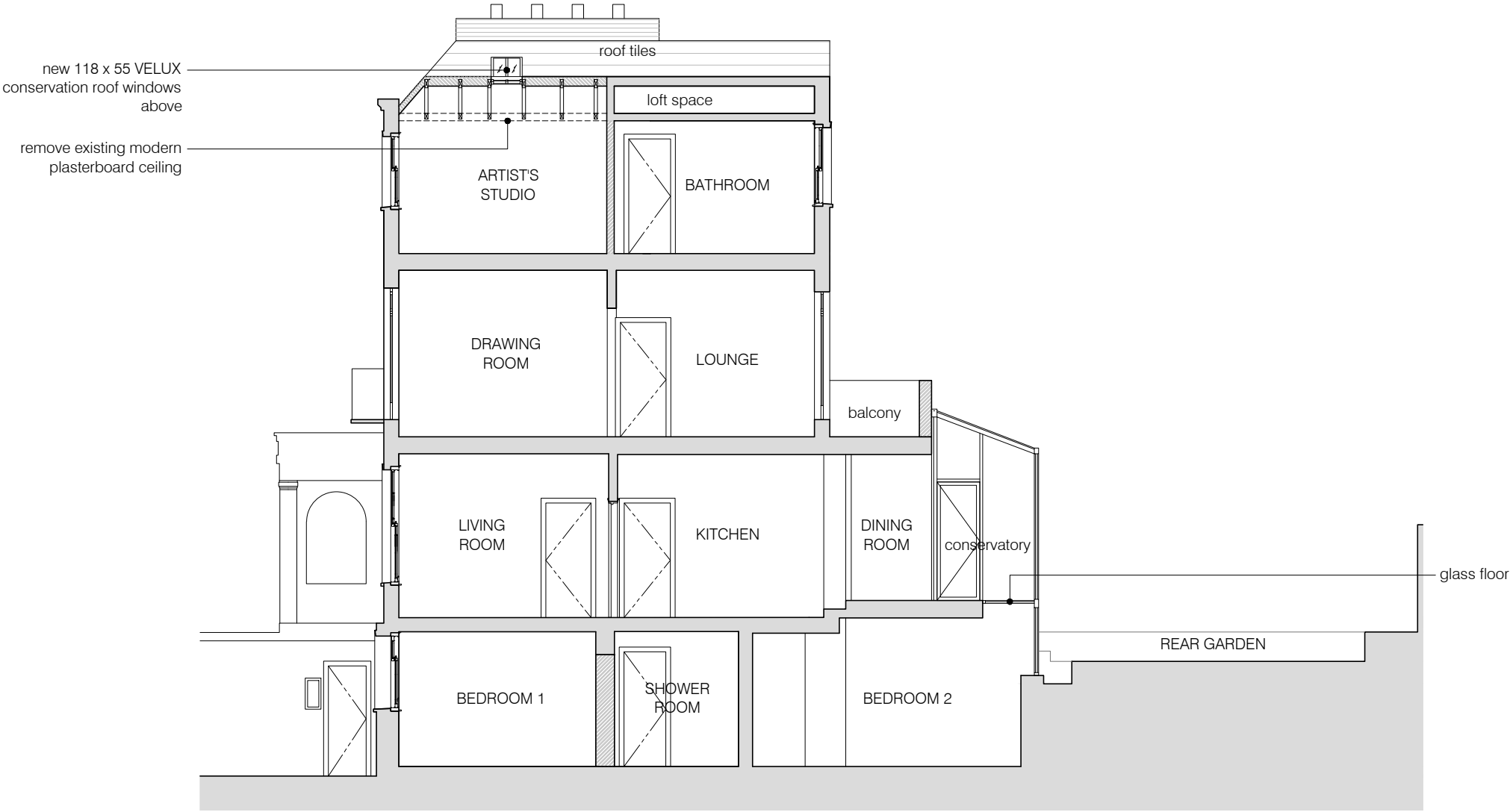
01 PROPOSED SECTION B-B scale 1:100
