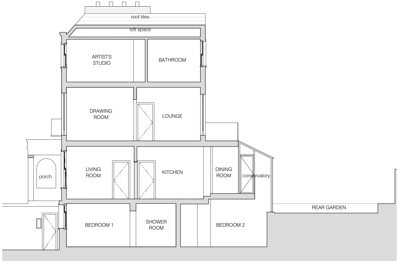
01 EXISTING SECTION B-B scale 1:100
