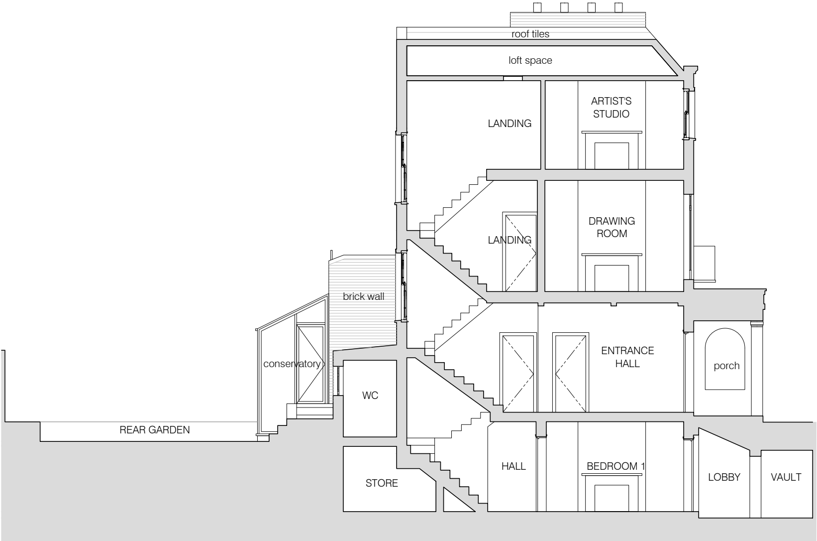
01 EXISTING SECTION A-A scale 1:100
