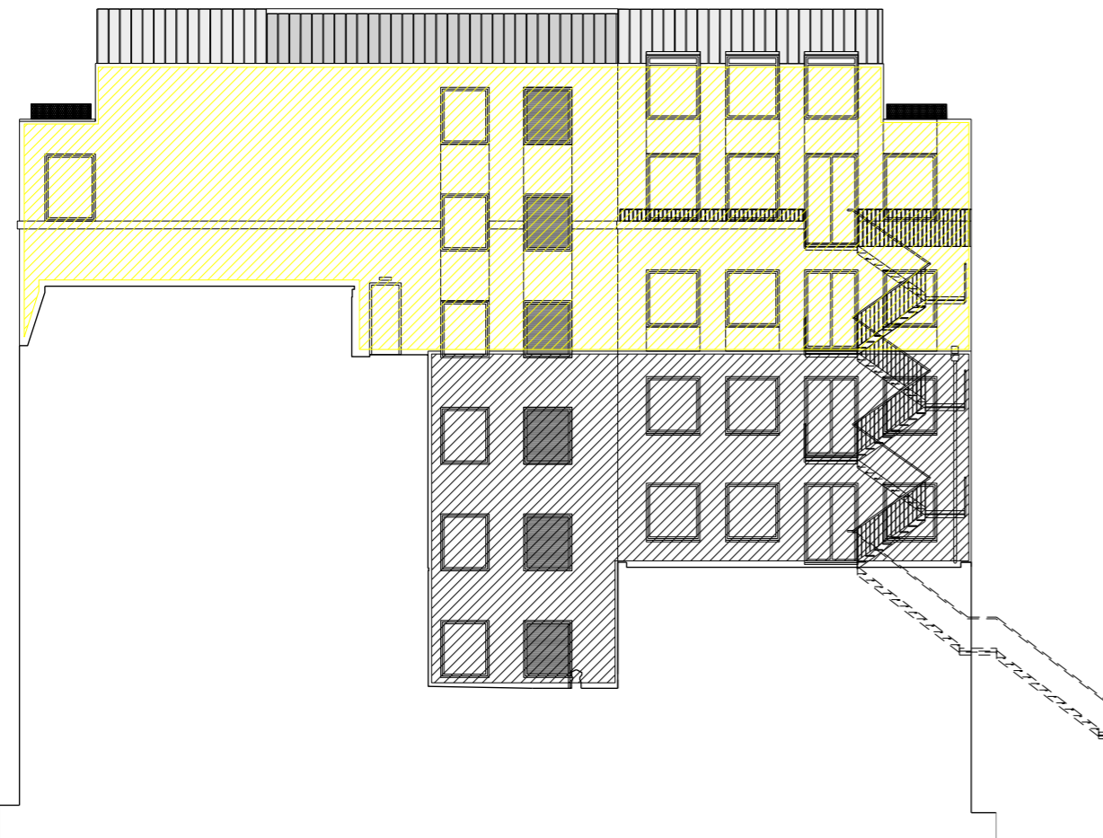
03 Elevation 3 - Proposed PL_265 Brick Types 1:100
