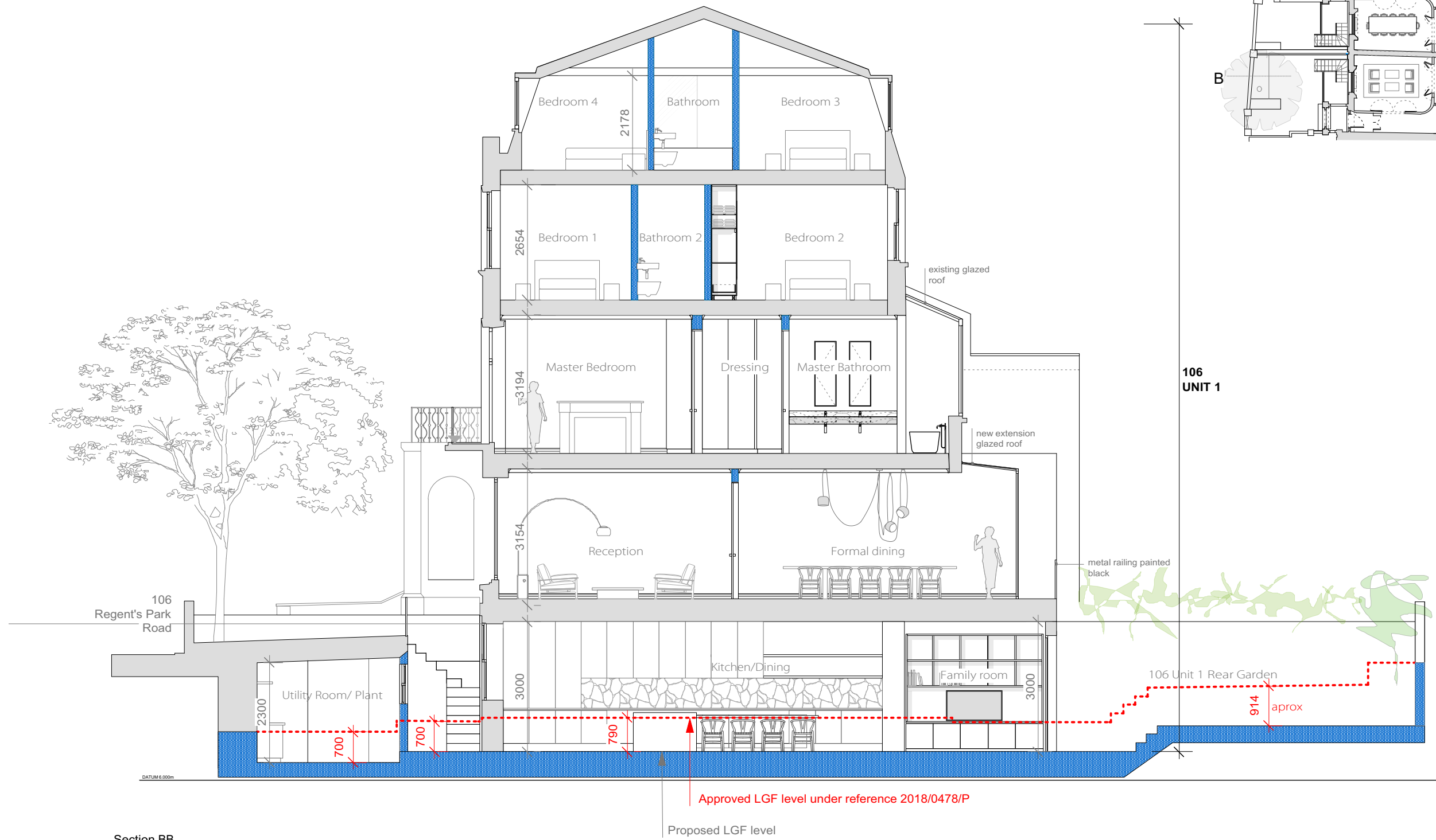
Section BB
