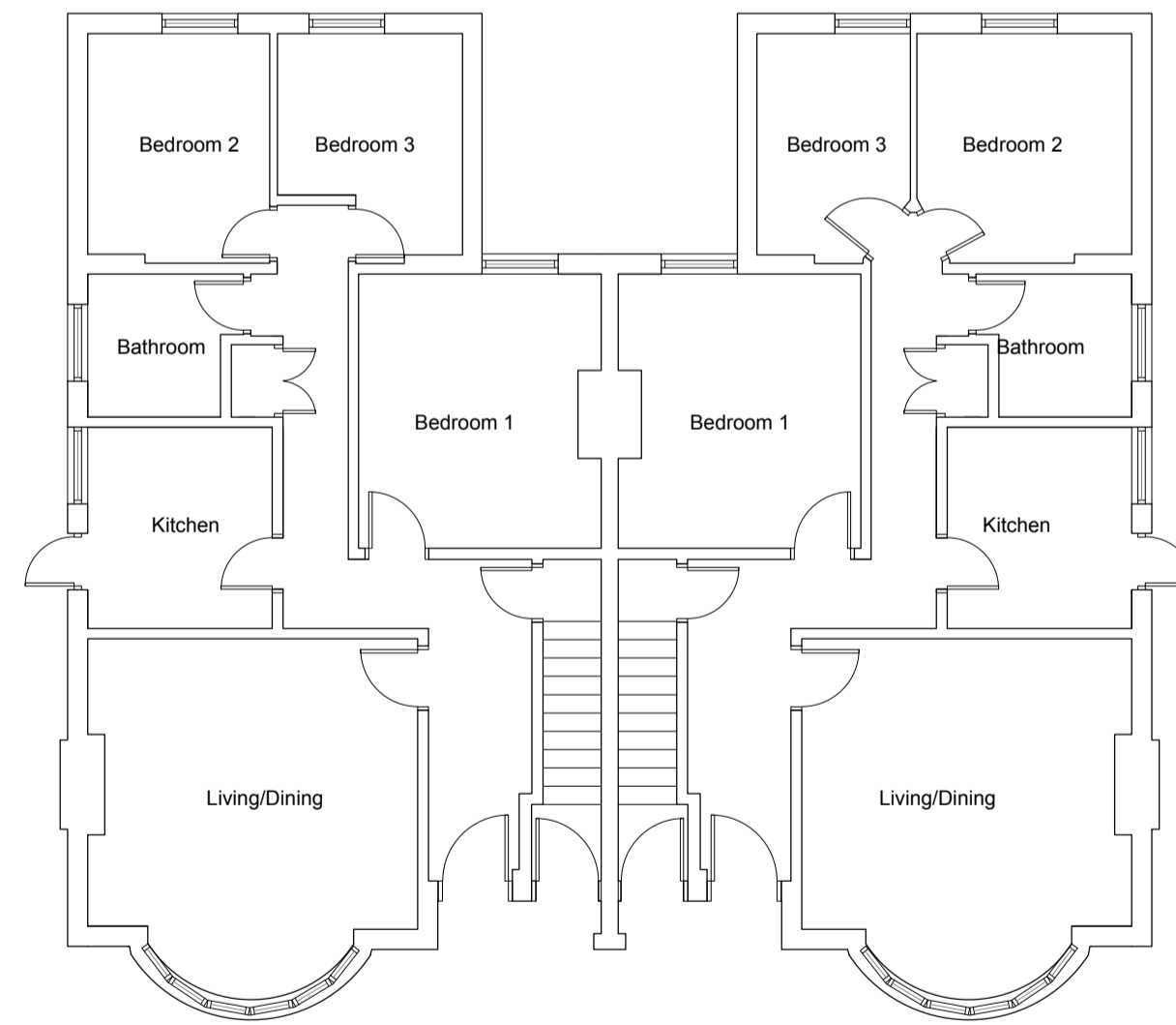
① Existing Ground Floor Plan 1:100
