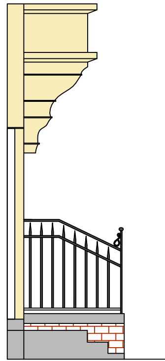
Existing Side Elevation - C
