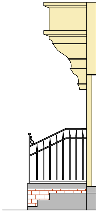
Existing Side Elevation - B
