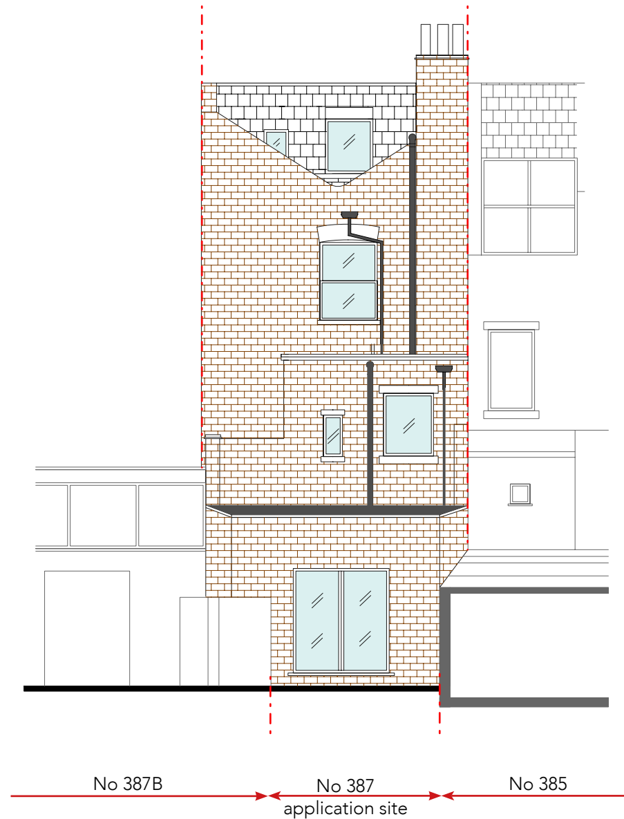
Existing Rear Elevation (B)
