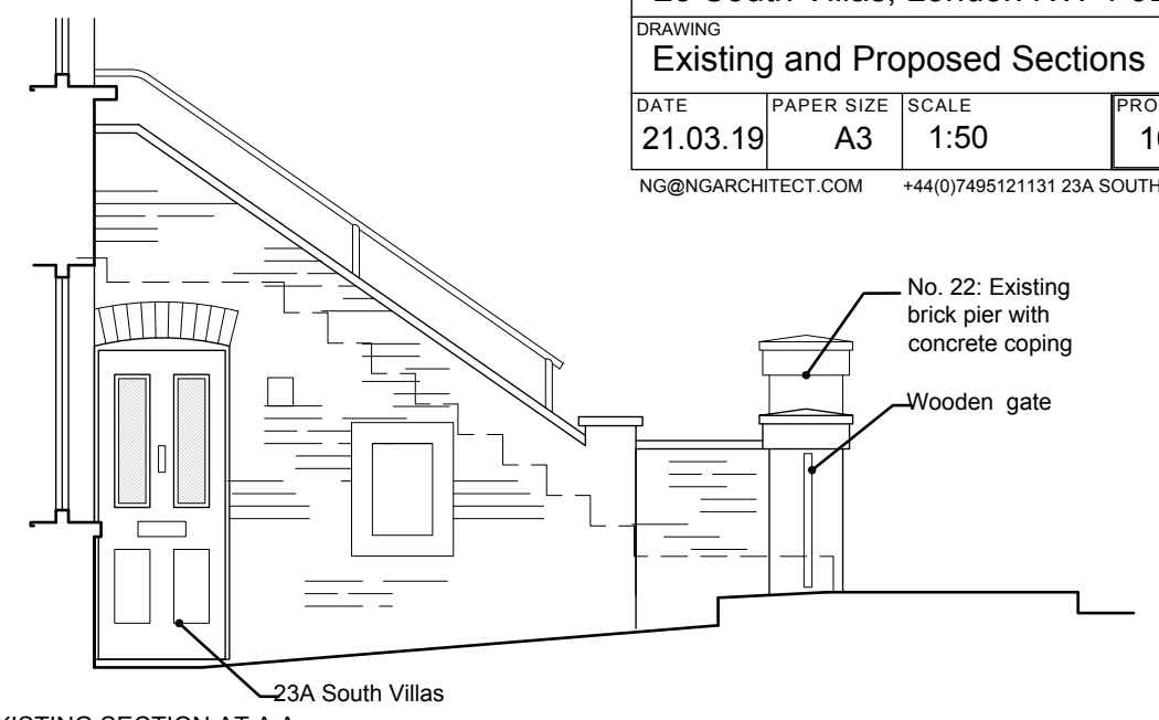
EXISTING SECTION AT A:A Scale 1:50
