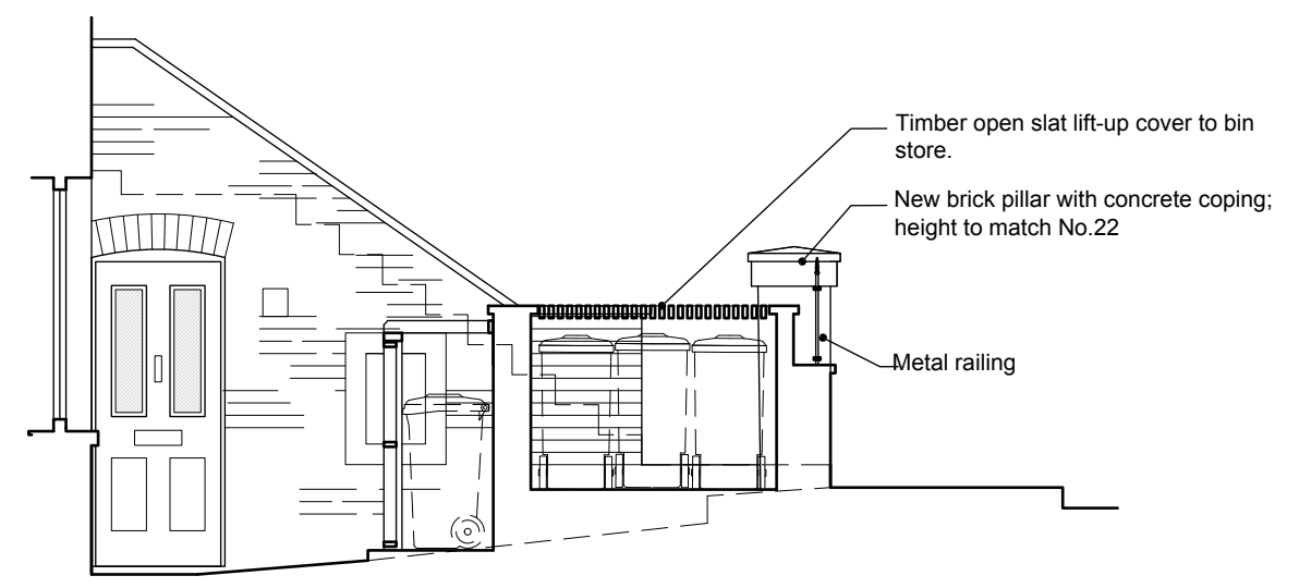
PROPOSED SECTION AT A:A Scale 1:50
