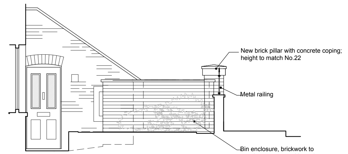
PROPOSED SECTION AT B:B Scale 1:50
