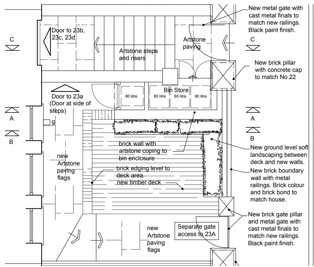
PROPOSED PLAN - LOCATION OF SECTIONS Scale 1:50
