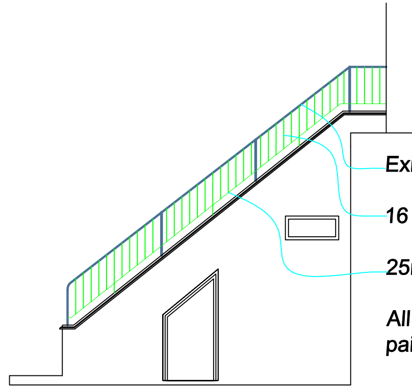
Proposed Elevation
