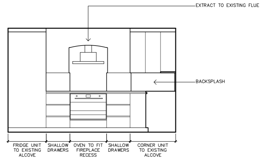
PROPOSED SOUTH-EAST KITCHEN ELEVATION
