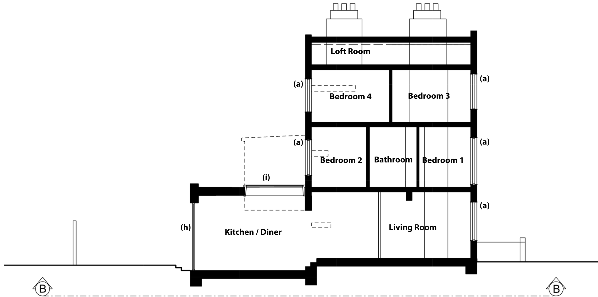
SECTION B
